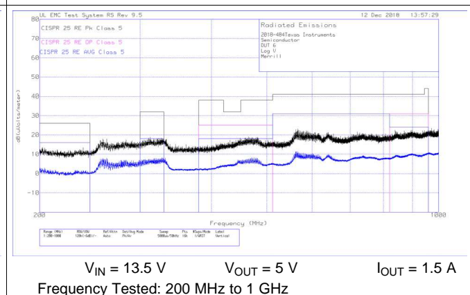
图 38. Radiated EMI Log Vertical vs. CISPR25 Limits
