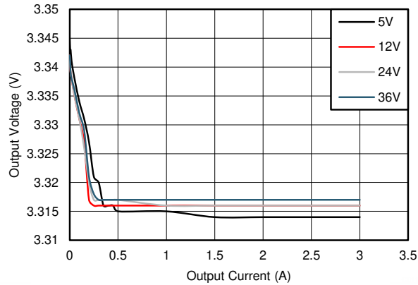
图 9-25. Line and Load Regulation
