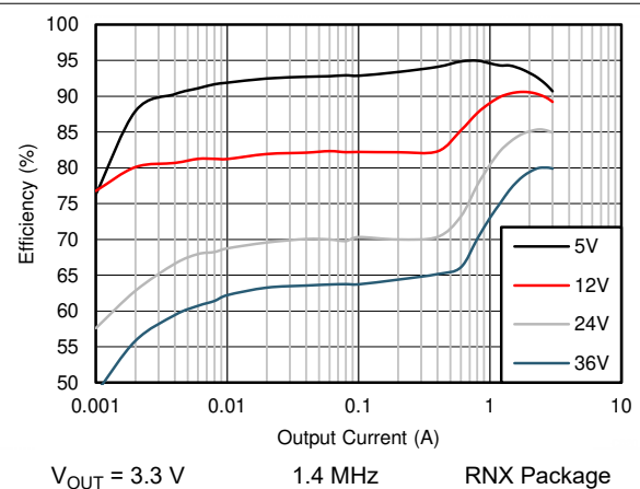
图 9-16. Efficiency
