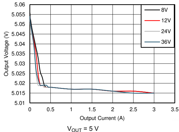
图 9-19. Line and Load Regulation
