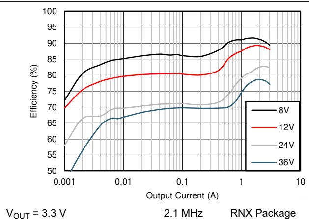
图 9-18. Efficiency
