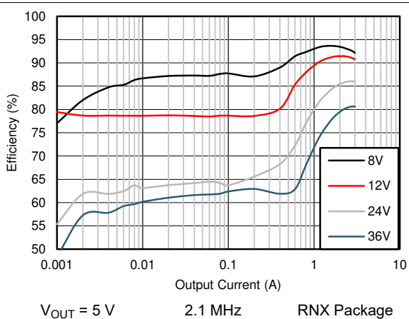
图 9-17. Efficiency
