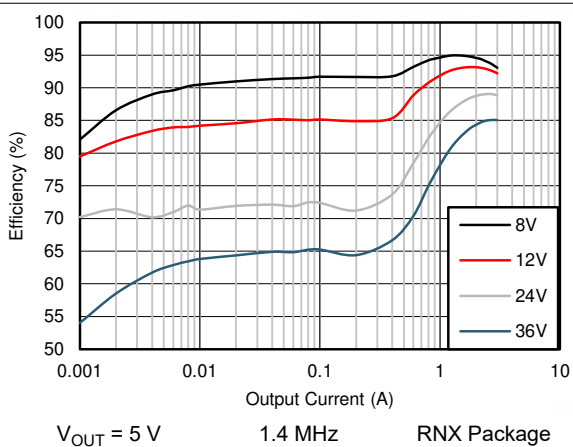
图 9-15. Efficiency
