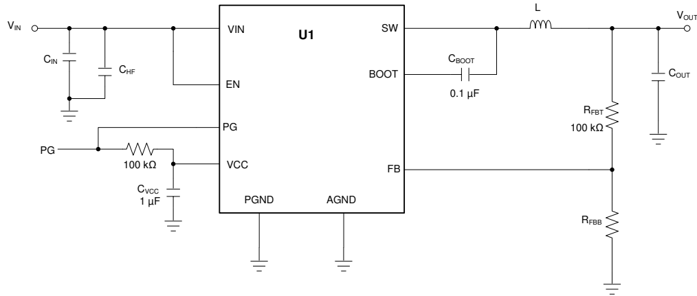
图 8-35. Circuit for Application Curves
