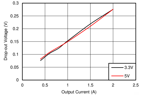
图 7-10. Typical Dropout Voltage versus Output Current in Frequency Foldback f_{SW} = 140\text{ kHz}
