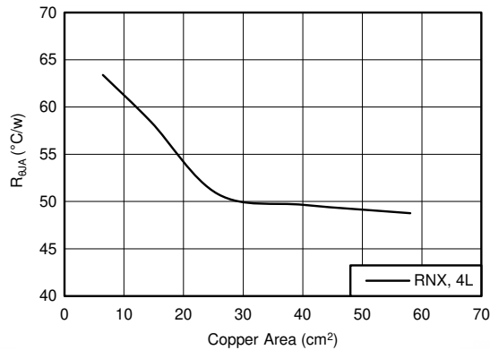
图 8-7. R_{\theta JA} versus Copper Board Area for the VQFN (RNX) Package
