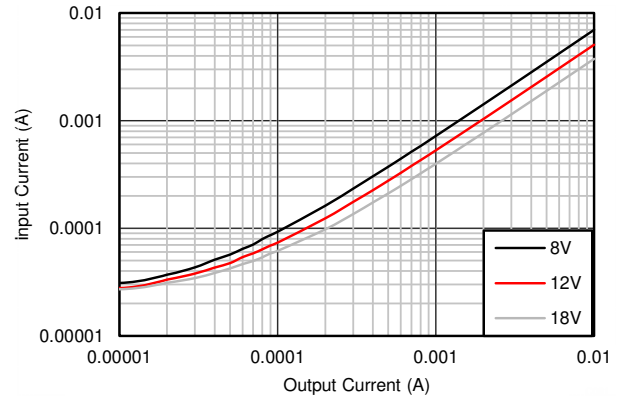
图 8-3. Input Supply Current vs Output Current for 5-V Fixed Output Option
