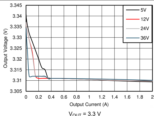
图 8-23. Line and Load Regulation
