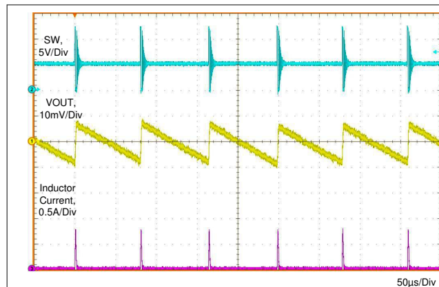
图 7-7. Typical PFM Switching Waveforms V_{IN} = 12 V, V_{OUT} = 5 V, I_{OUT} = 10 mA
