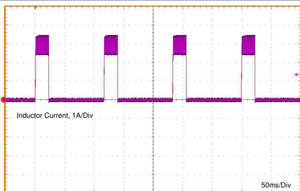
图 7-5. Inductor Current Burst in Short-Circuit Mode
