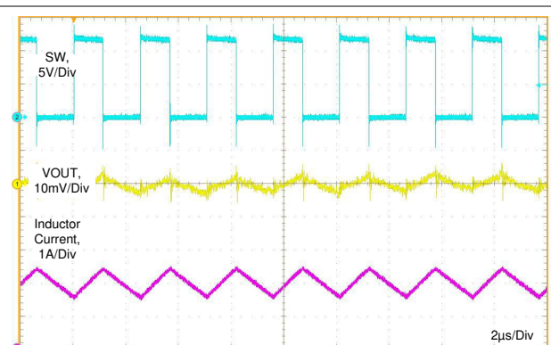
图 7-8. Typical PWM Switching Waveforms V_{IN} = 12 V, V_{OUT} = 5 V, I_{OUT} = 2 A, f_S = 400 kHz
