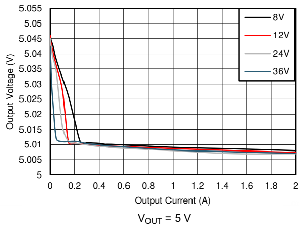
图 8-17. Line and Load Regulation
