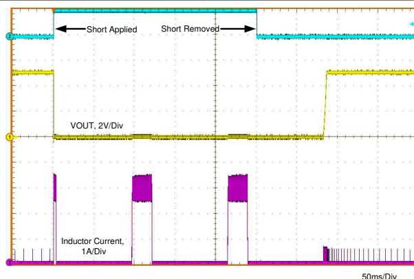
图 7-6. Short-Circuit Transient and Recovery
