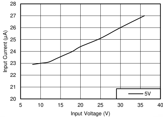
图 8-2. No-load Input Supply Current for 5-V Fixed Output Option
