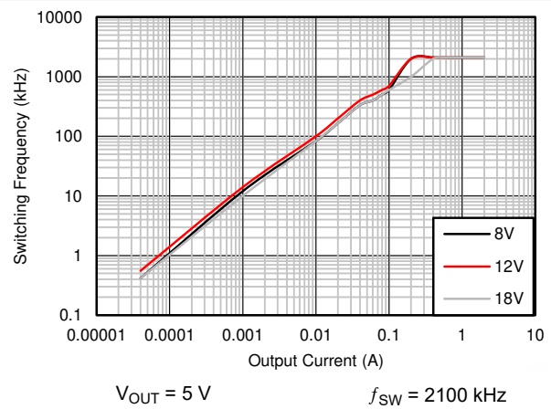
图 8-20. Switching Frequency versus Output Current
