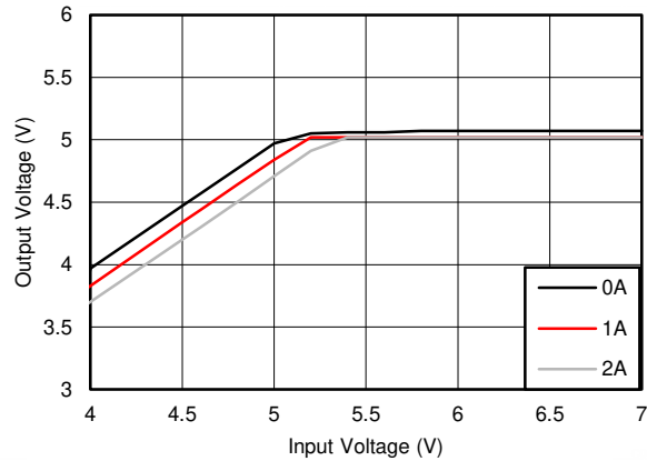
图 7-9. Overall Dropout Characteristic V_{OUT} = 5\text{ V}
