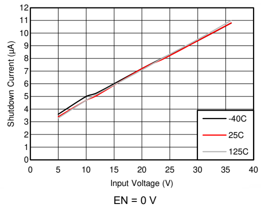
图 6-2. Shutdown Supply Current
