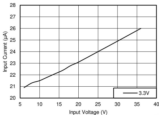
图 8-4. No-load Input Supply Current for 3.3-V Fixed Output Option
