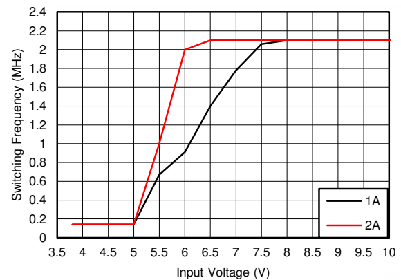
图 7-12. Typical Switching Frequency in Dropout Mode V_{OUT} = 5\text{ V} , f_{SW} = 2.1\text{ MHz}
