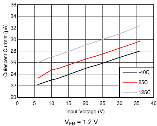
图 6-1. Non-Switching Input Supply Current
