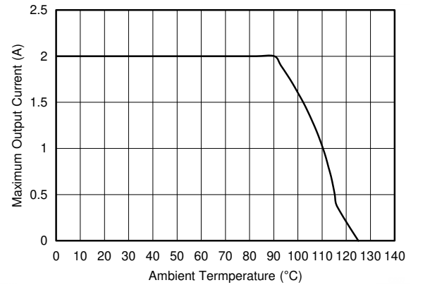
图 8-8. Maximum Output Current versus Ambient Temperature
