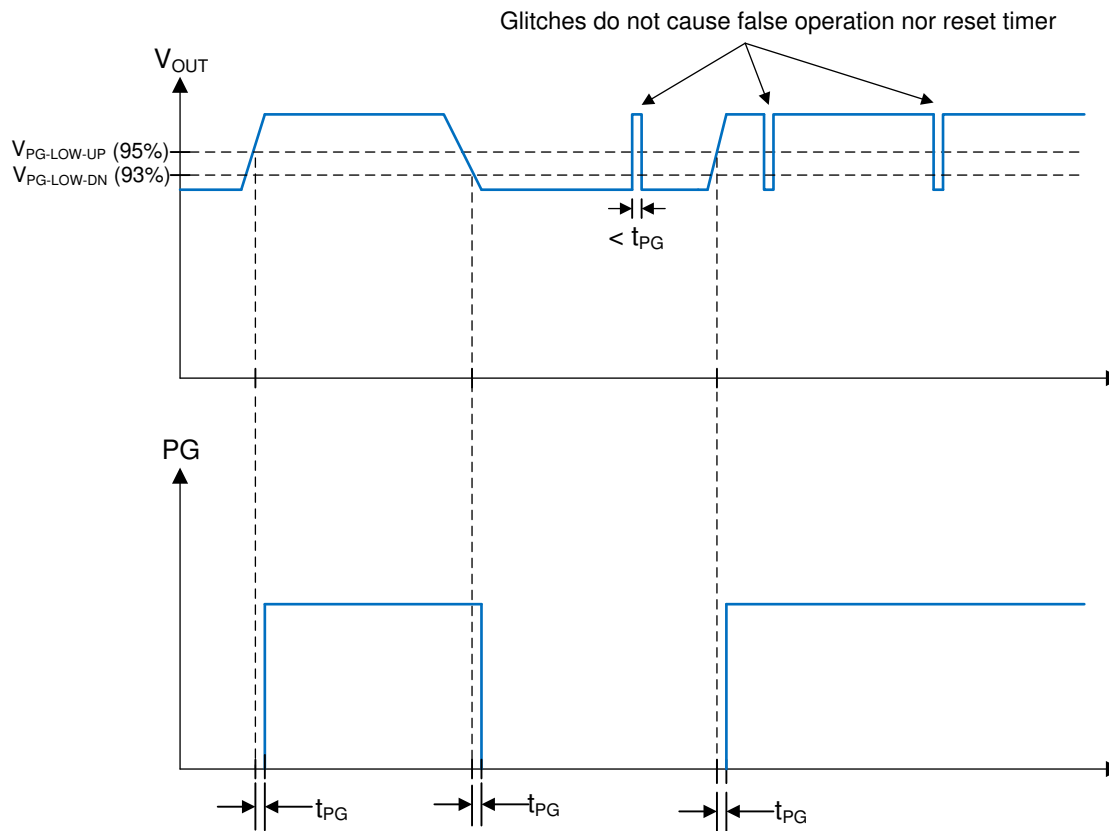
图 7-2. Power-Good-Timing Behavior
