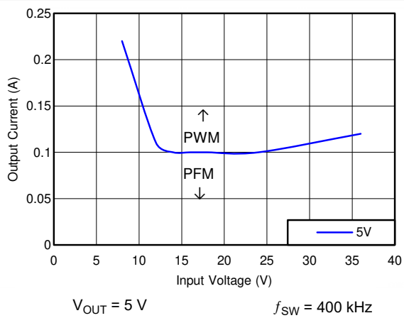
图 8-19. Mode Change Thresholds
