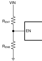
图 8-6. Setup for External UVLO Application
