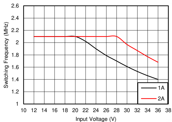
图 7-13. Switching Frequency versus Input Voltage V_{OUT} = 3.3\text{ V}
