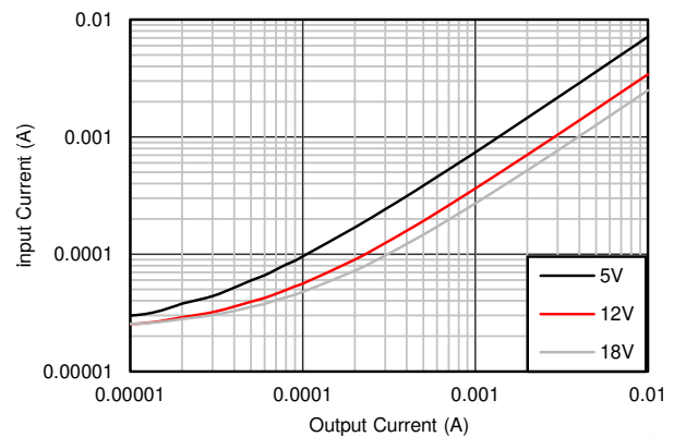
图 8-5. Input Supply Current vs Output Current for 3.3-V Fixed Output Option
