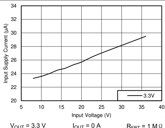
图 8-24. Input Supply Current
