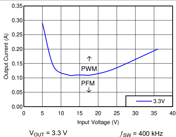
图 8-25. Mode Change Thresholds
