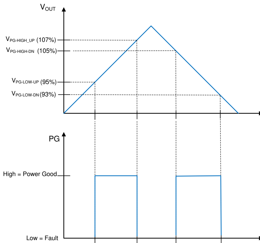
图 7-1. Static Power-Good Operation
