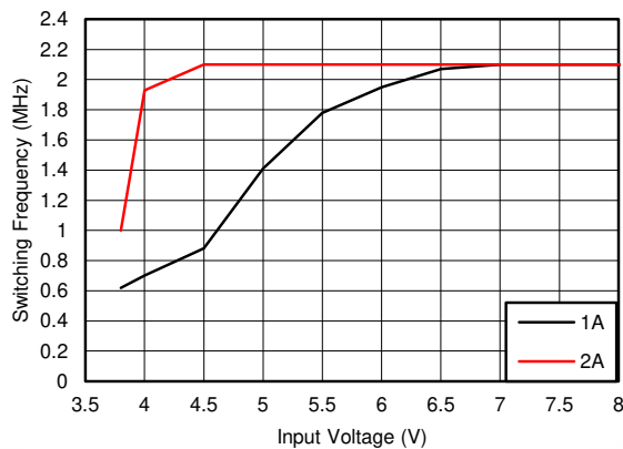
图 7-11. Typical Switching Frequency in Dropout Mode V_{OUT} = 3.3\text{ V} , f_{SW} = 2.1\text{ MHz}
