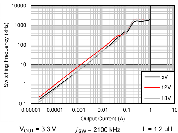
图 8-26. Switching Frequency versus Output Current
