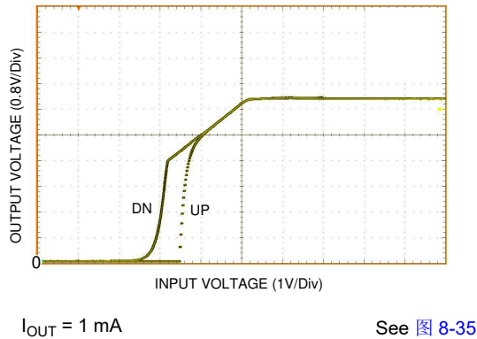
图 6-5. UVLO Thresholds
