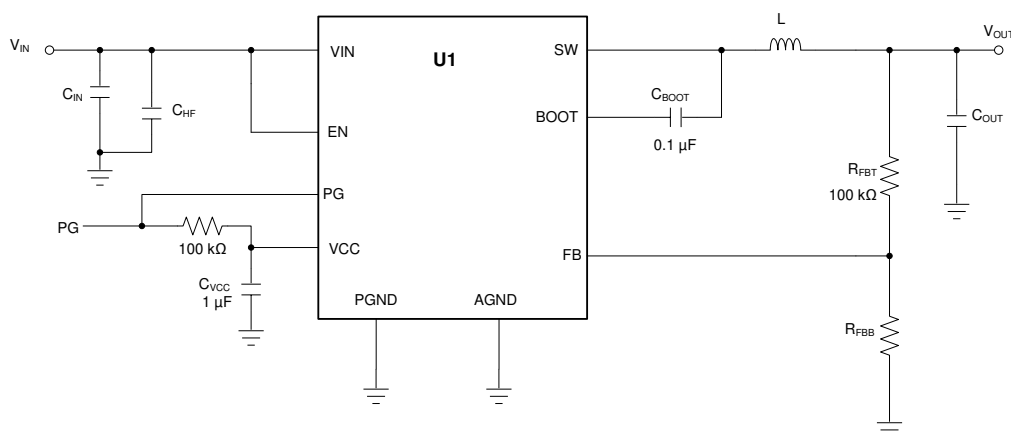
图 9-20. Circuit for Application Curves
