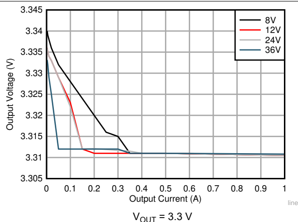
图 9-11. Line and Load Regulation
