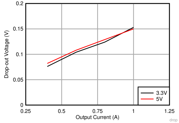
图 8-10. Typical Dropout Voltage vs Output Current in Frequency Foldback, f_{SW} = 140\text{ kHz}
