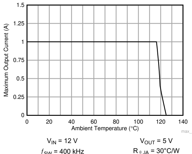
Figure 9-4. Maximum Output Current vs Ambient Temperature
