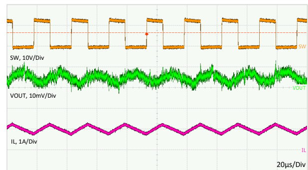
图 8-8. Typical PWM Switching Waveforms, V_{IN} = 12 V, V_{OUT} = 5 V, I_{OUT} = 1 A, f_s = 400 kHz
