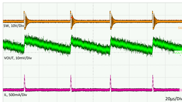
图 8-7. Typical PFM Switching Waveforms, V_{IN} = 12 V, V_{OUT} = 5 V, I_{OUT} = 10 mA
