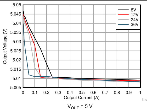
图 9-10. Line and Load Regulation
