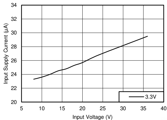
图 9-13. Input Supply Current
