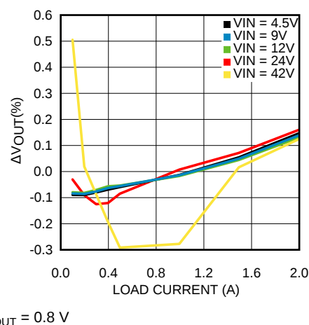
Figure 10. V_{OUT} Regulation vs Load Current
