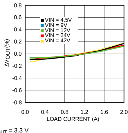
Figure 8. V_{OUT} Regulation vs Load Current
