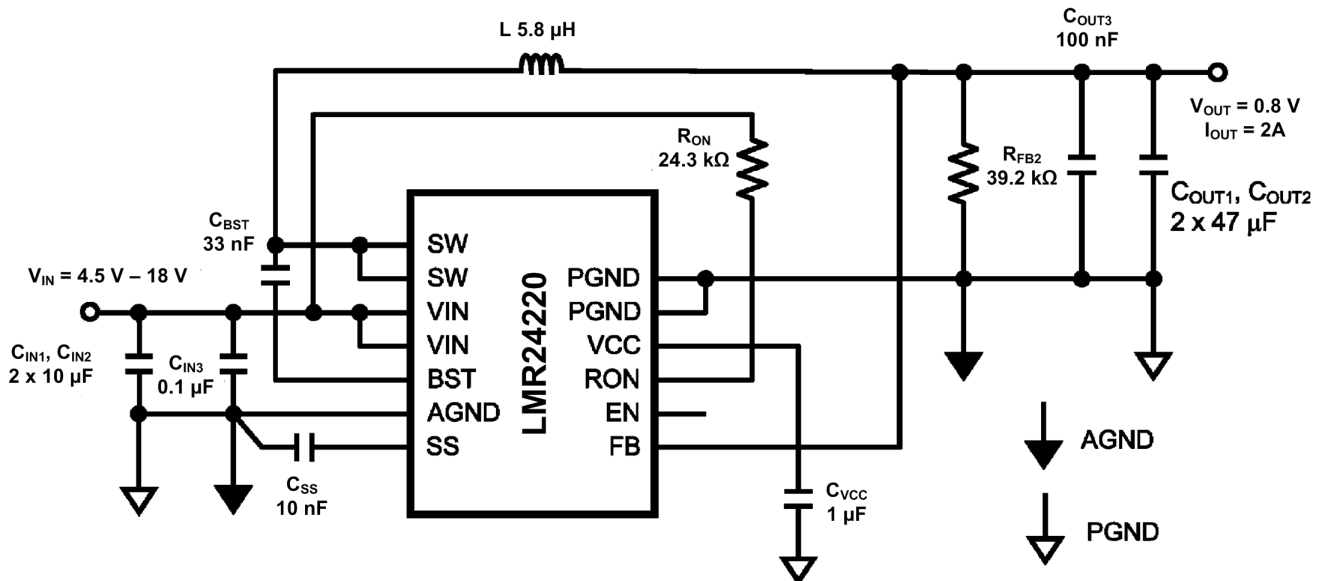
Figure 26. Typical Application Schematic For V_{OUT} = 0.8\text{ V}
