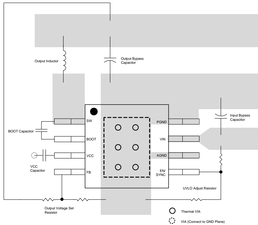
Figure 34. SOIC Layout
