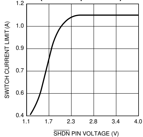
Switch Current Limit vs. \overline{\text{SHDN}} Pin Voltage (Soft-Start Implementation)
