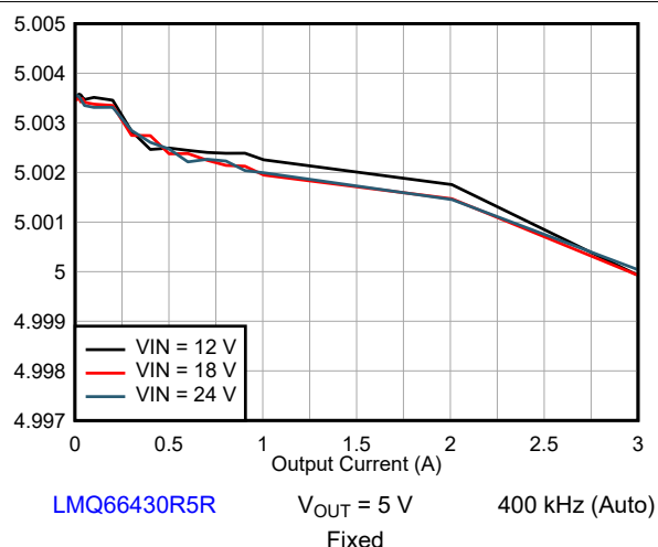
图 9-7. Line and Load Regulation
