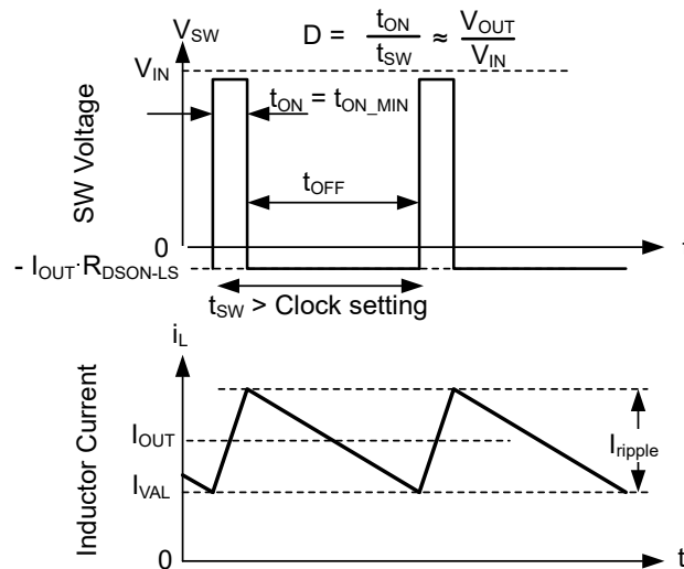
图 8-17. Valley Current Mode Operation
