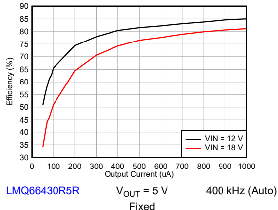
图 9-5. Efficiency
