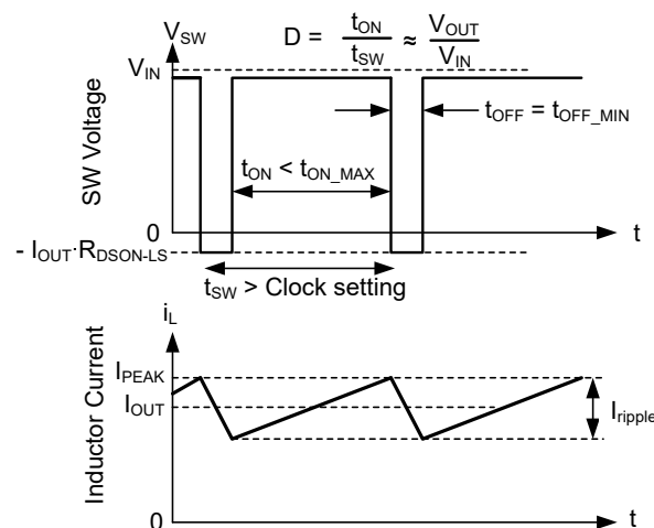
图 8-18. Frequency and Output Voltage in Dropout
