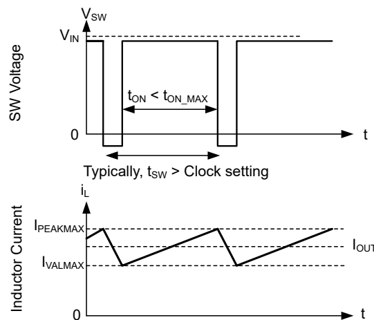
图 8-10. Current Limit Waveforms
