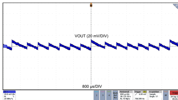
LMQ66430R5R V_{OUT} = 5\text{ V} 0 A Load Fixed
