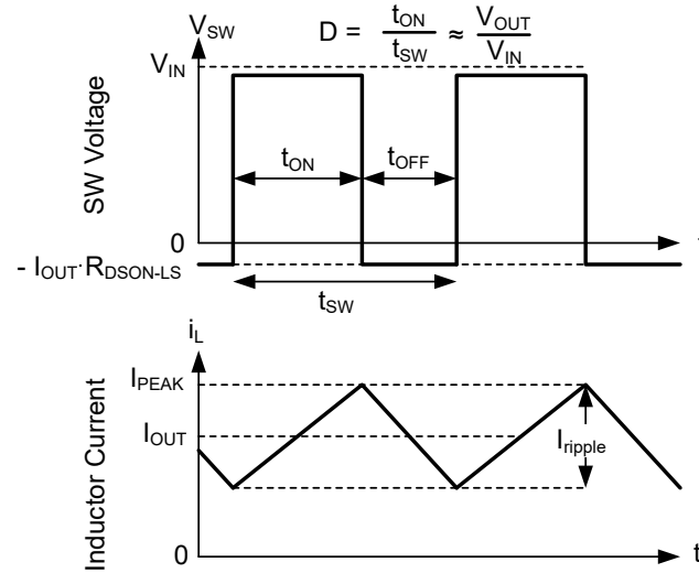
图 8-13. SW Voltage and Inductor Current Waveforms in Continuous Conduction Mode (CCM)
