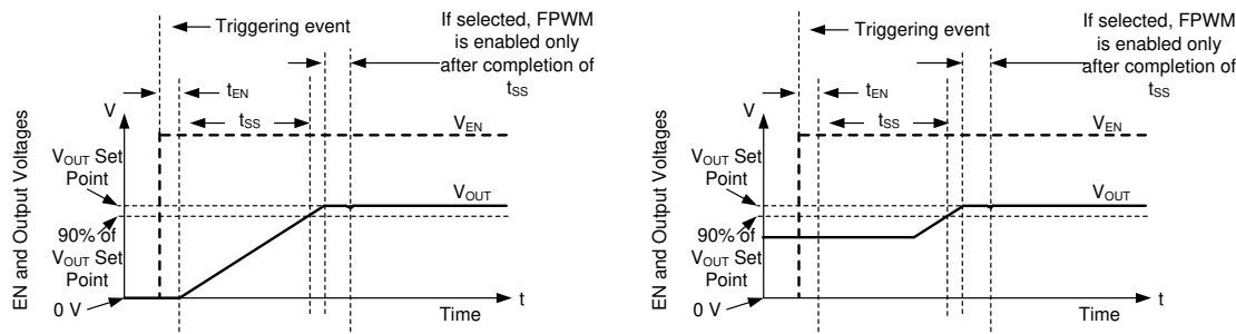
图 8-7. Soft Start with and Without Pre-bias Voltage
