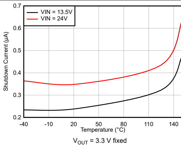
图 7-1. Shutdown Current Versus Temperature
