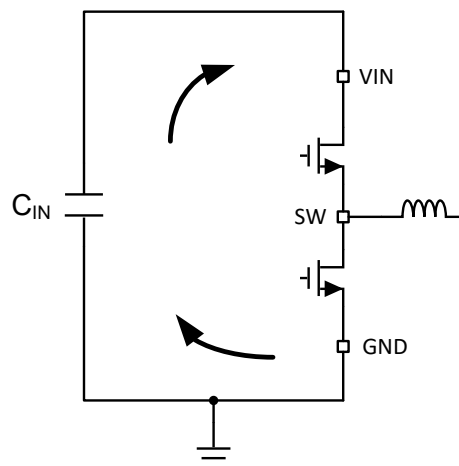
图 9-12. Current Loops with Fast Edges
