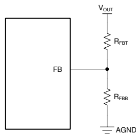
图 8-6. Setting Output Voltage for Adjustable Output Variant
