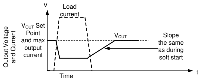
图 8-8. Recovery from Dropout
