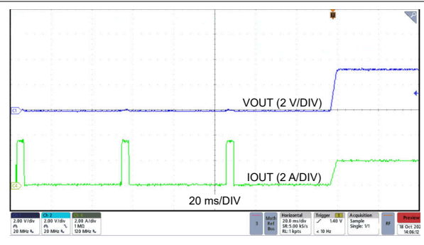
图 8-12. Hiccup Exit
