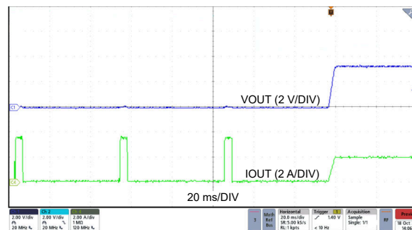
图 8-12. Hiccup Exit
