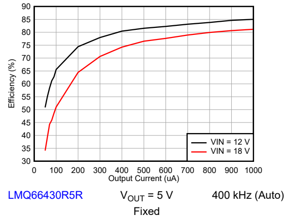
图 9-5. Efficiency
