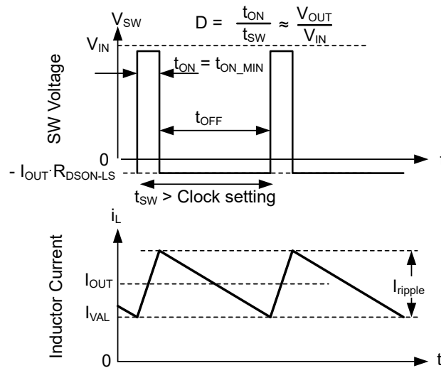
图 8-17. Valley Current Mode Operation
