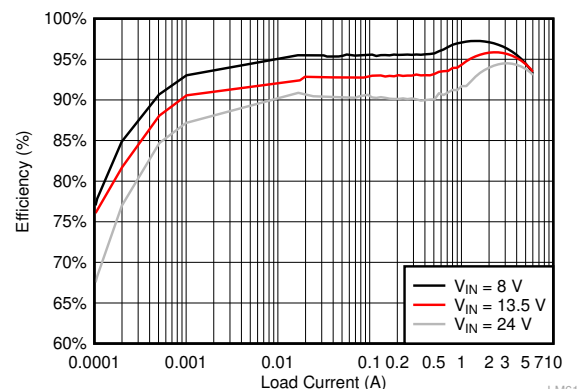
效率：V OUT =5V，f sw =400 kHz
