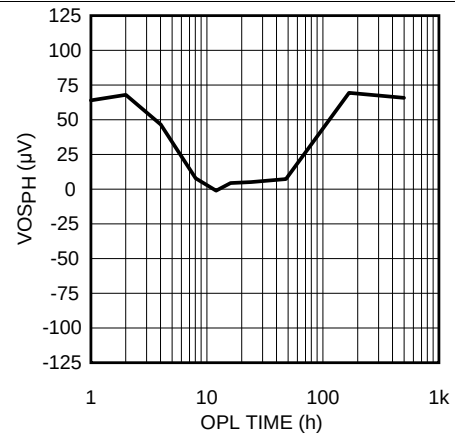
Figure 14. pH Buffer Input Offset Voltage Drift
