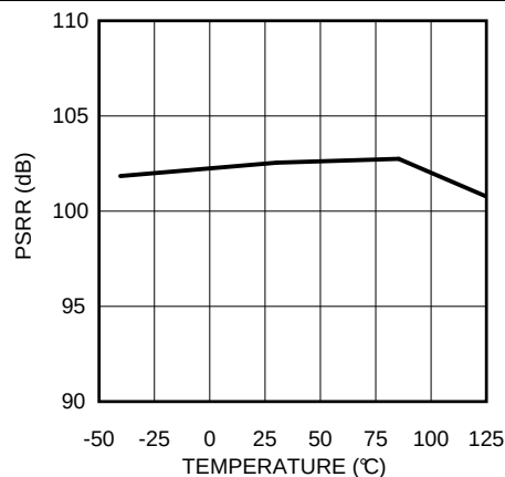
Figure 24. VCM Buffer DC PSRR vs Temperature
