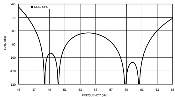
Figure 43. Digital Filter Response at 13.42 SPS
