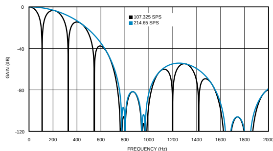
Figure 45. Digital Filter Response 107.325 SPS and 214.65 SPS
