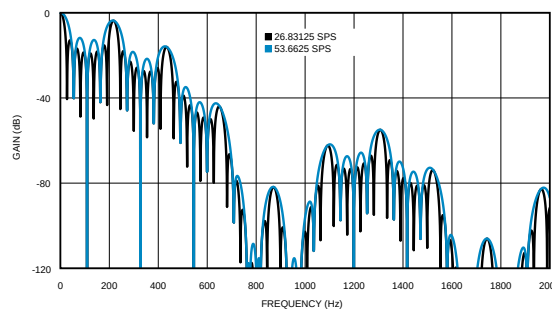
Figure 44. Digital Filter Response, 26.83125 SPS and 53.6625 SPS
