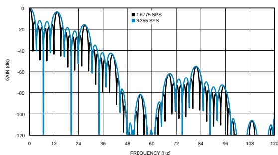
Figure 41. Digital Filter Response, 1.6775 SPS and 3.355 SPS
