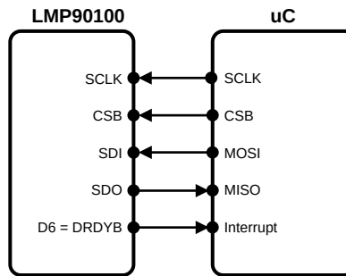
Figure 63. DRDYB Case3 Connection Diagram
