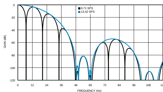
Figure 42. Digital Filter Response, 6.71 SPS and 13.42 SPS
