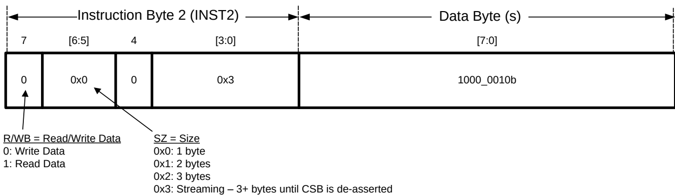
Figure 71. Setting up SPI_STREAMCN
