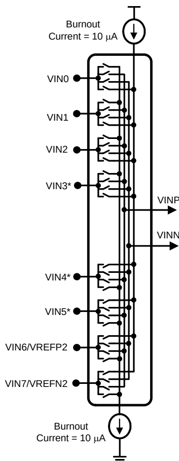
Figure 52. Burnout Currents
