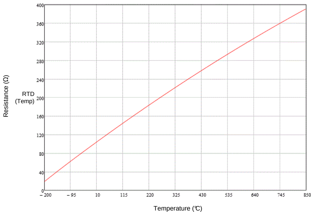
Figure 75. PT-100 RTD Resistance from –200°C to 850°C
