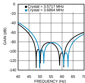
Figure 46. Digital Filter Response for a 3.5717 MHz versus 3.6864 MHz XTAL
