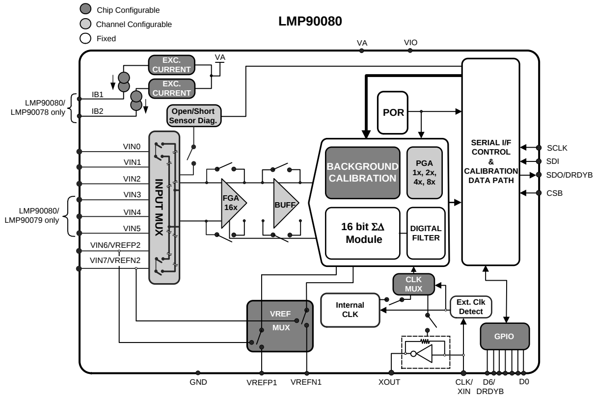
Figure 1. Block Diagram
