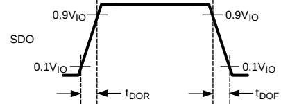
Figure 11. SDO Rise and Fall Time
