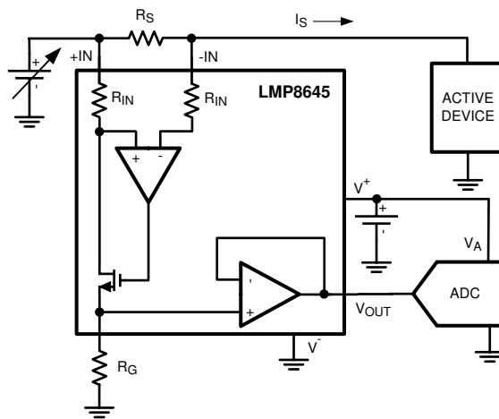
图 8-1. LMP8645 in Current Monitor Application
