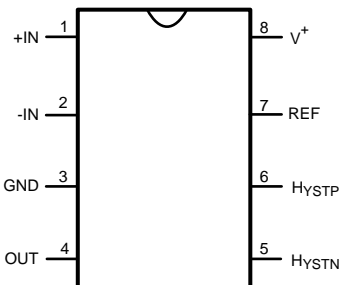
Pin Functions
