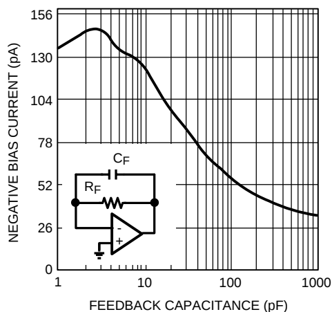
Figure 42. Input Bias Current vs. C_F with R_F = 1 G \Omega
