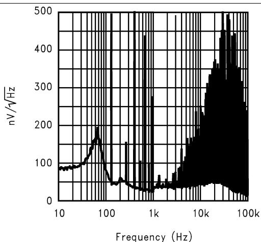
Figure 28. The Output of a Chopper Stabilized Op Amp (MAX432)
