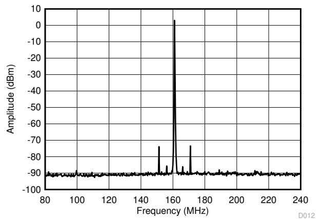
图 6-10. 161.1328125 ± 80.56640625-MHz LVPECL Differential Output Spectrum
