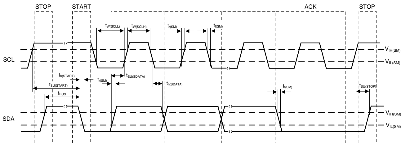
图 8-5. I 2 C Timing Diagram
