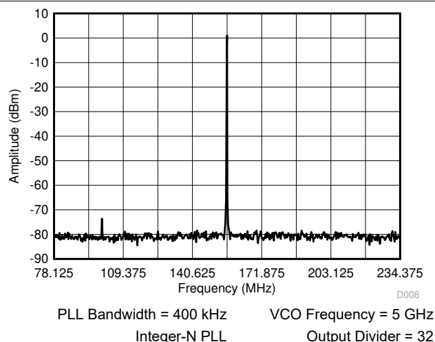
图 6-8. 156.25 ± 78.125-MHz LVDS Differential Output Spectrum
