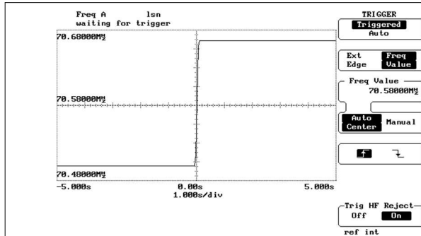
图 9-2. Increasing Output Frequency in DCXO Mode
