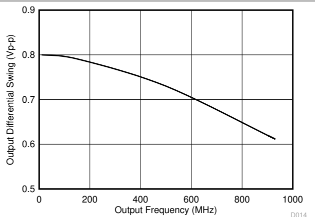
图 6-14. LVDS Differential Output Swing vs Frequency
