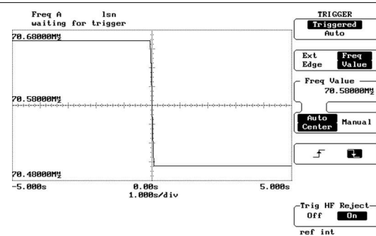
图 9-3. Decreasing Output Frequency in DCXO Mode
