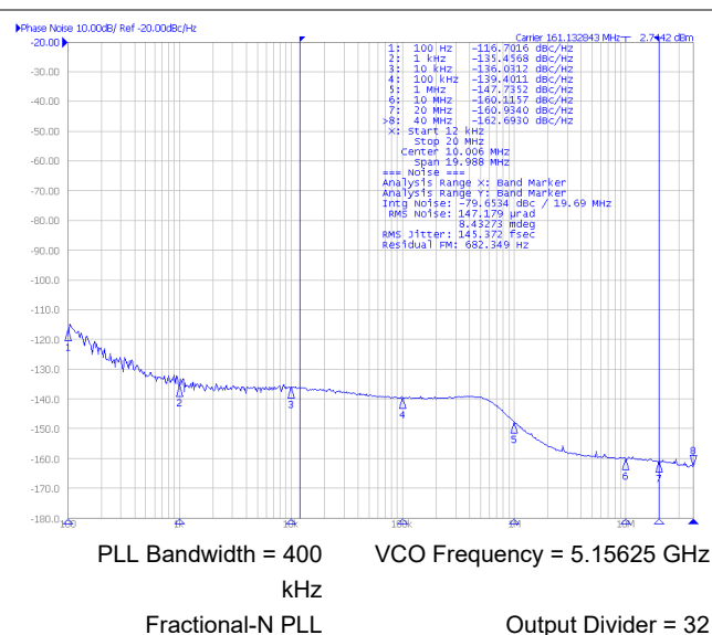
图 6-6. Closed-Loop Phase Noise of HCSL Differential Output at 161.1328125 MHz
