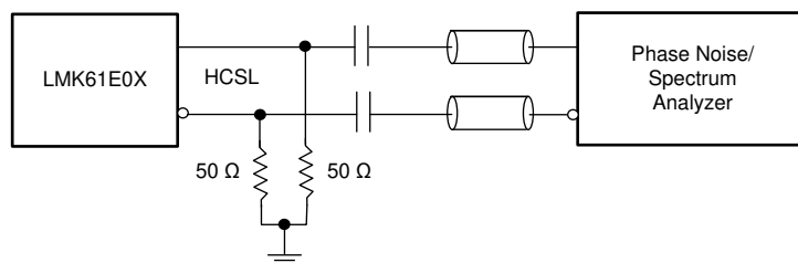
图 7-5. LVDS Output AC Configuration During Device Test
