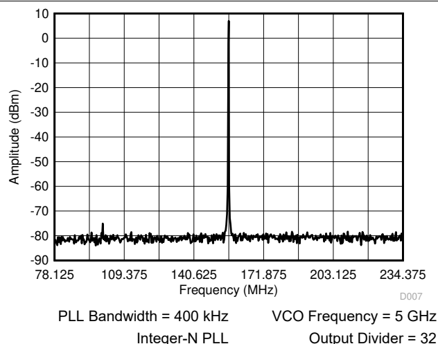
图 6-7. 156.25 ± 78.125-MHz LVPECL Differential Output Spectrum
