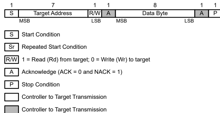
图 8-7. Generic Programming Sequence
