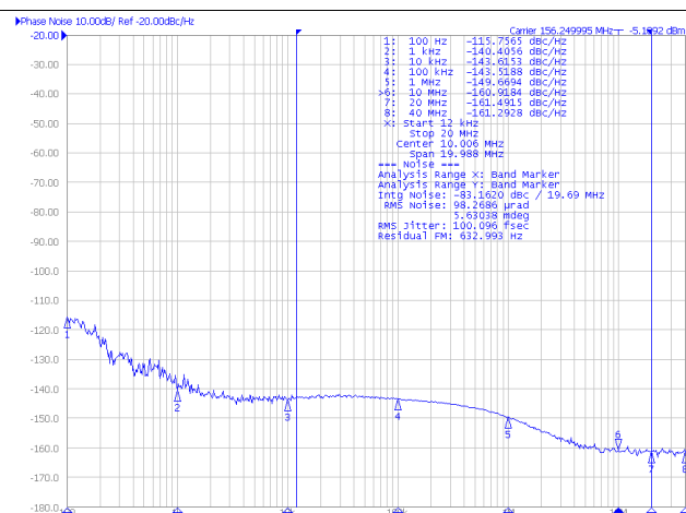
Figure 2. Phase Noise of 156.25-MHz LVDS Differential Output
