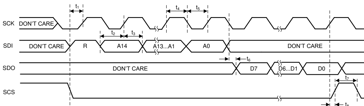
图 7-2. SPI 4-Wire Read Timing Diagram
