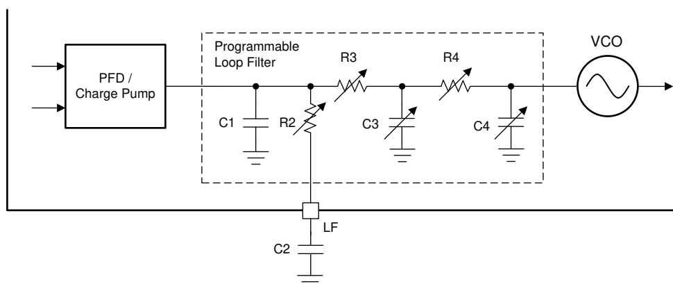
图 9-24. Loop Filter Structure of Each APLL
