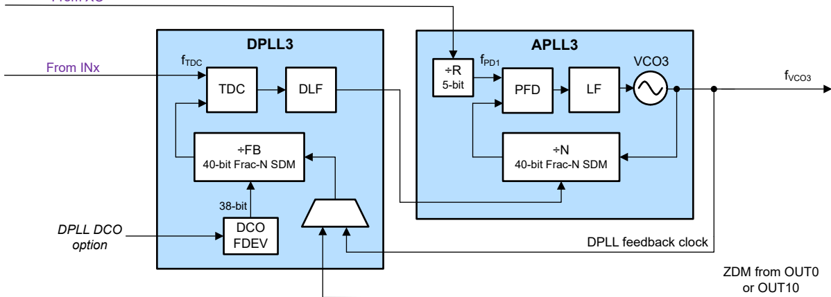
图 9-5. APLL Cascaded with DPLLs Enabled Example
