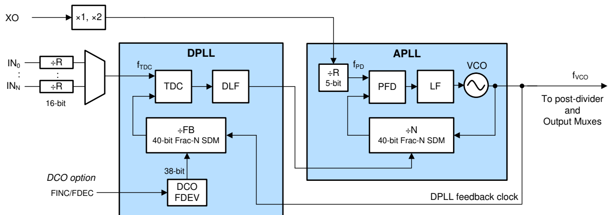
图 9-23. PLL Architecture
