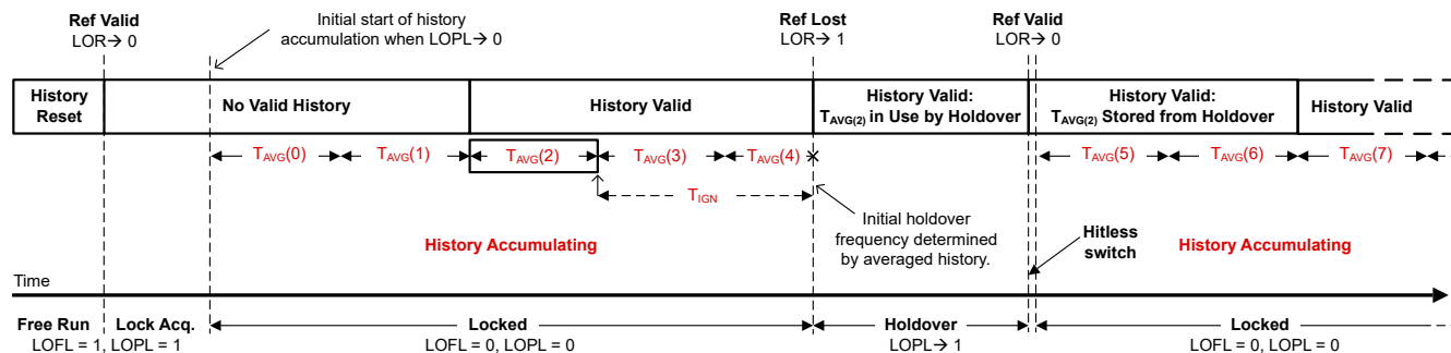
图 9-21. Tuning Word History Windows
