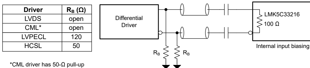
图 9-15. AC-Coupled Differential to Reference (INx)
