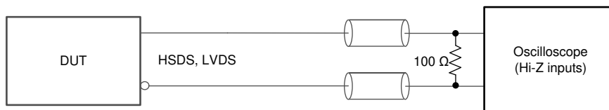
图 8-5. HSDS, LVDS Output DC Test Configuration
