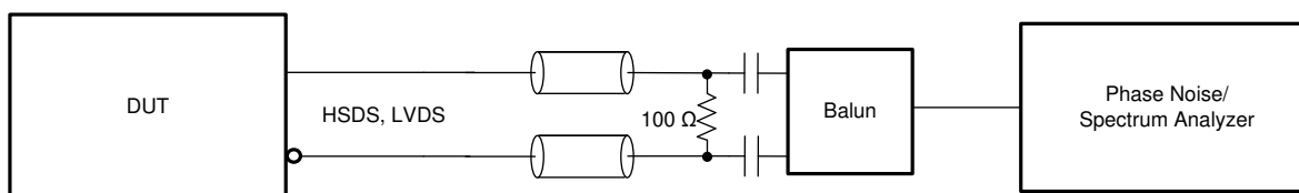
图 8-6. HSDS, LVDS Output Phase Noise Test Configuration
