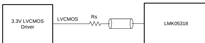
图 30. Single-Ended LVCMOS (1.8, 2.5, 3.3 V) to Reference (PRIREF_P/SECREP_P)
