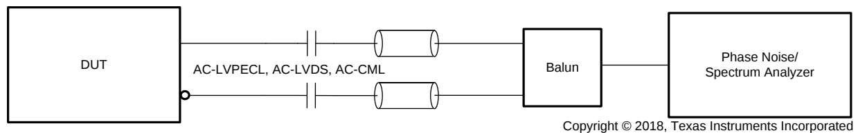
图 18. AC-LVPECL, AC-LVDS, AC-CML Output Phase Noise Test Configuration
