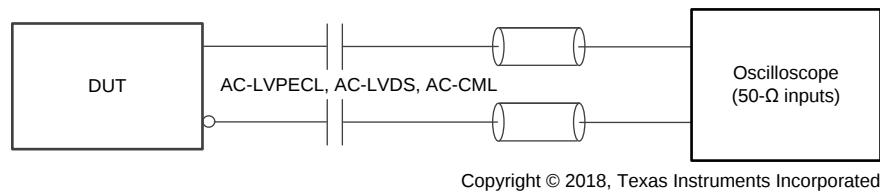
图 17. AC-LVPECL, AC-LVDS, AC-CML Output AC Test Configuration
