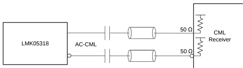
图 49. AC-CML Output to CML Receiver With Internal Termination/Biasing
