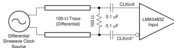
图 9-3. CLKinX/X* or OSCin Termination for a Differential Sinewave Reference Clock Source
