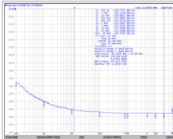
图 35. OSCout, 122.88 MHz, LVCMOS (Norm/Inv) Normal Output Measured, Inverse 50- \Omega Termination
