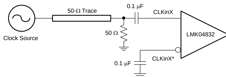
图 24. CLKinX/X* Single-Ended Termination
