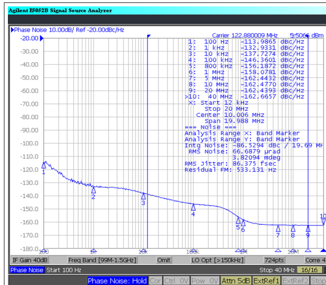
图 33. CLKout3 = 122.88 MHz, VCO = 2949.12 MHz CLKout2_3_IDL = 1, CLKout2_3_ODL = 1 With 120- \Omega Emitter Resistors
