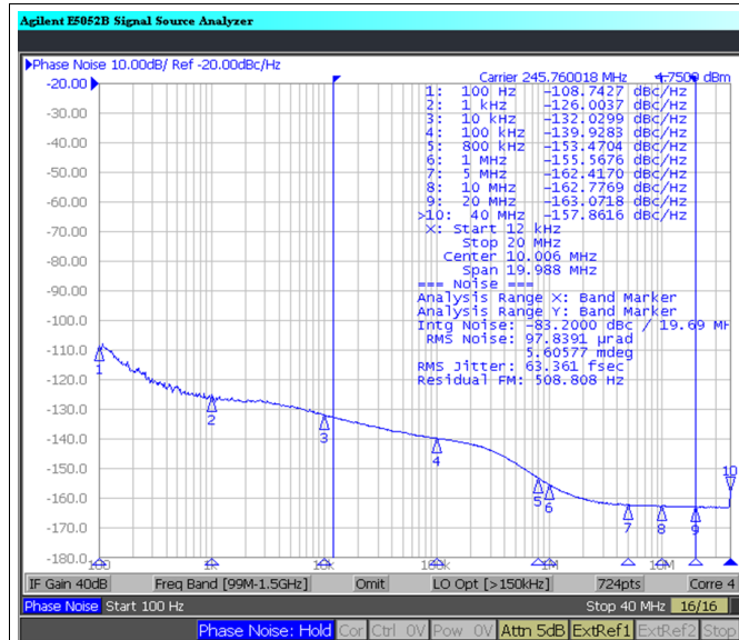
图 27. CLKout0 = 245.76 MHz, VCO = 2457.6 MHz CLKout0_1_IDL = 1, CLKout0_1_ODL = 1 LVPECL20 With 240- \Omega Emitter Resistors
