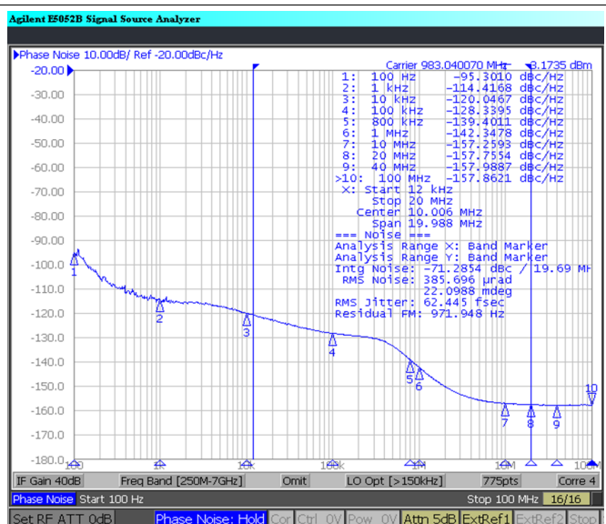
图 30. CLKout2 = 983.04-MHz, VCO = 2949.12 MHz CLKout2_3_IDL = 1, CLKout2_3_ODL = 1 LVPECL16 With 120- \Omega Emitter Resistors
