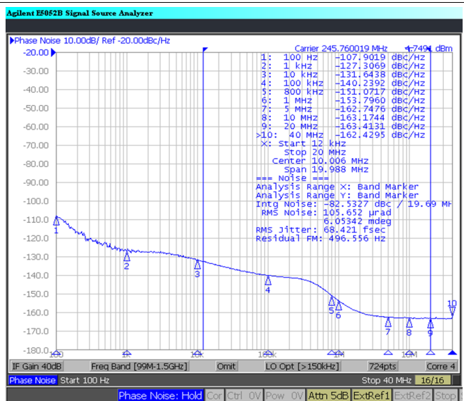
图 28. CLKout0 = 245.76 MHz, VCO = 2459.12 MHz CLKout0_1_IDL = 1, CLKout0_1_ODL = 1 LVPECL20 With 240- \Omega Emitter Resistors
