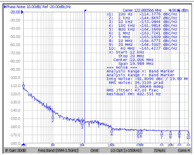
图 36. Direct VCXO Measurement Open-Loop, Holdover Mode Set
