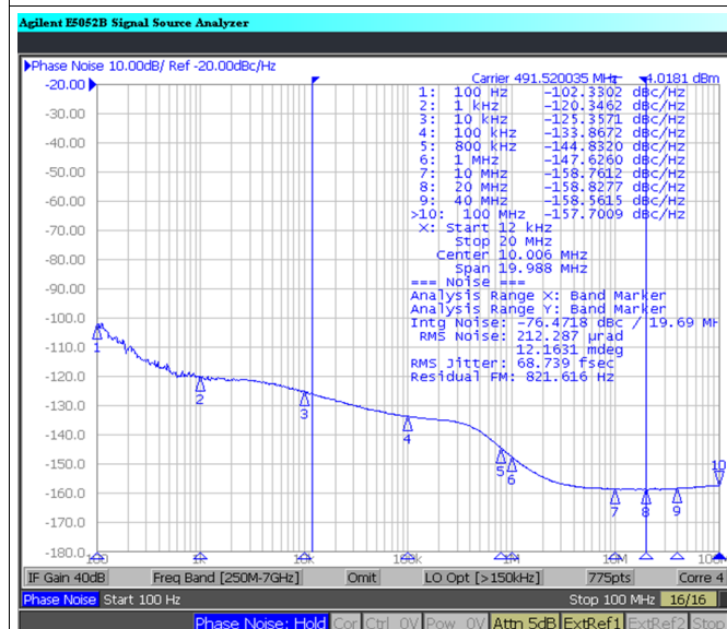
图 29. CLKout2 = 491.52-MHz, VCO = 2949.12 MHz CLKout2_3_IDL = 1, CLKout2_3_ODL = 1 LVPECL16 With 120- \Omega Emitter Resistors
