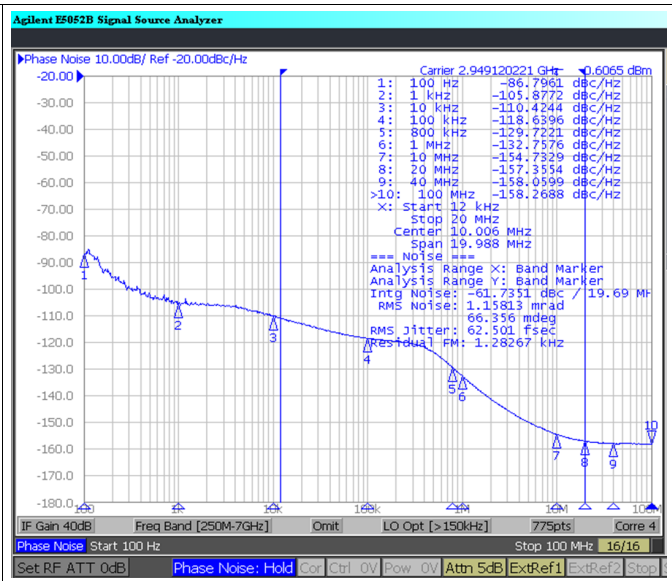
图 32. CLKout4 = 2949.12, VCO = 2949.12 MHz CLKout4_5_IDL = 1, CLKout4_5_ODL = 1 LVPECL, 68 nH Inductor - 20 \Omega Resistor
