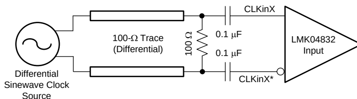
图 23. CLKInX/X* or OSCIn Termination for a Differential Sinewave Reference Clock Source
