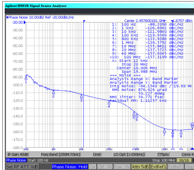
图 31. CLKout4 = 2457.6, VCO = 2457.6 MHz CLKout4_5_IDL = 1, CLKout4_5_ODL = 0 CML 32mA, 68 nH Inductor - 20 \Omega Resistor
