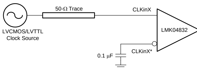
图 25. DC-Coupled LVCMOS/LVTTL Reference Clock
