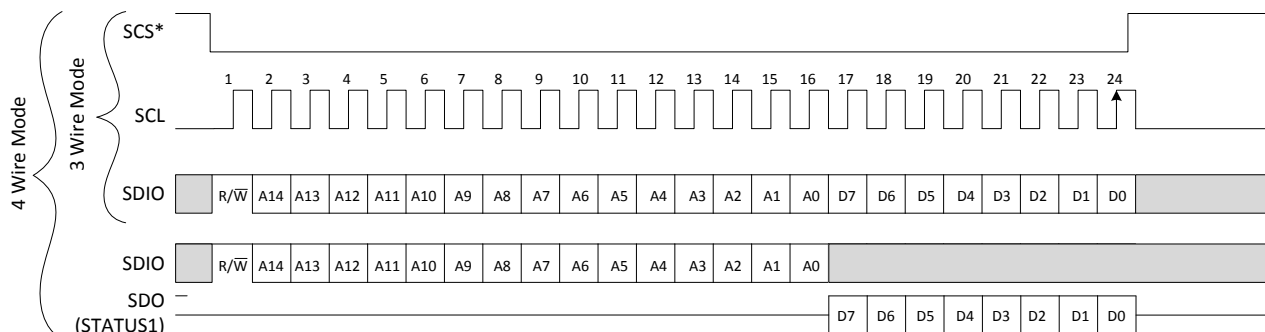
Figure 56. SPI Read
