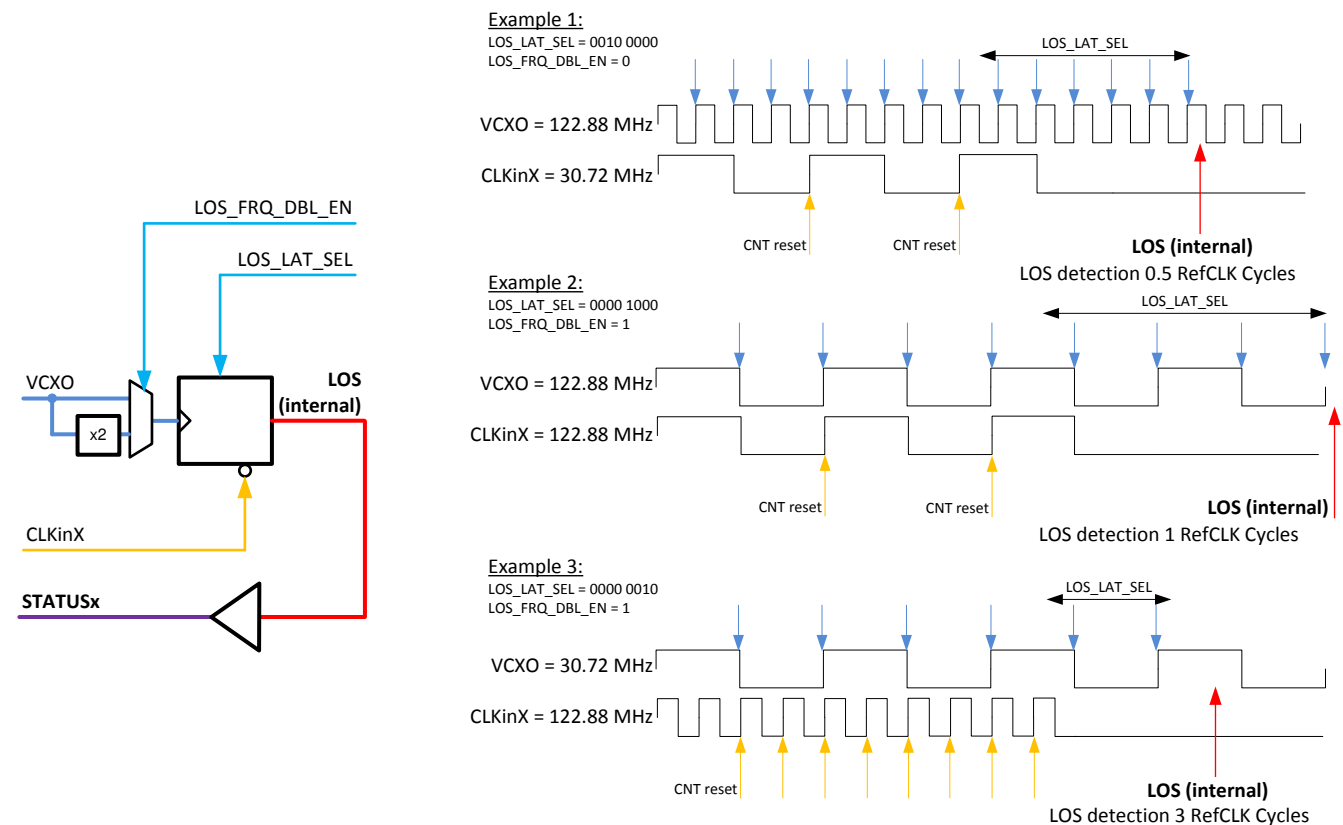
Figure 17. LOS Detection
