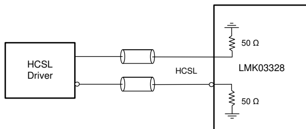
图 8-11. DC-Coupling LMK03328 Inputs With HCSL Signal
