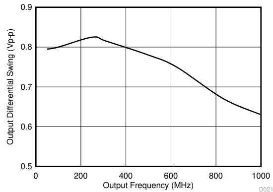
图 6-19. AC-LVDS Differential Output Swing vs. Frequency
