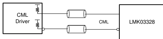
图 8-10. DC-Coupling LMK03328 Inputs With CML Signal
