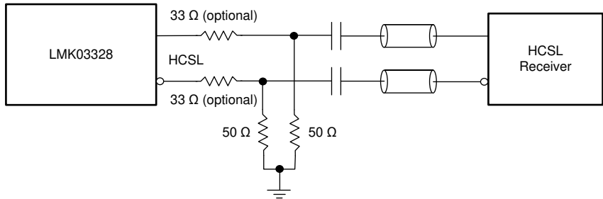
图 8-28. Interfacing the LMK03328 Output With HCSL Receiver
