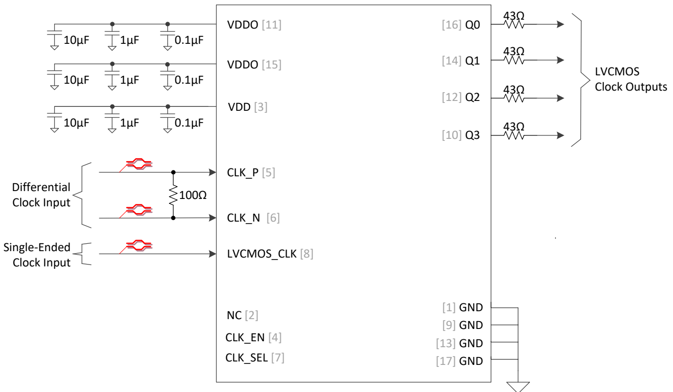
图 9. Typical Connection Diagram
