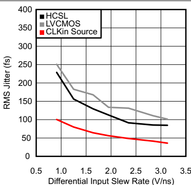
图 6-5. RMS Jitter vs CLKIn Slew Rate at 100 MHz
