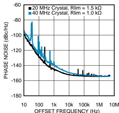
Figure 20. HCSL Phase Noise @ 100 MHz
