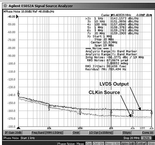
Figure 19. LVDS Phase Noise @ 100 MHz
