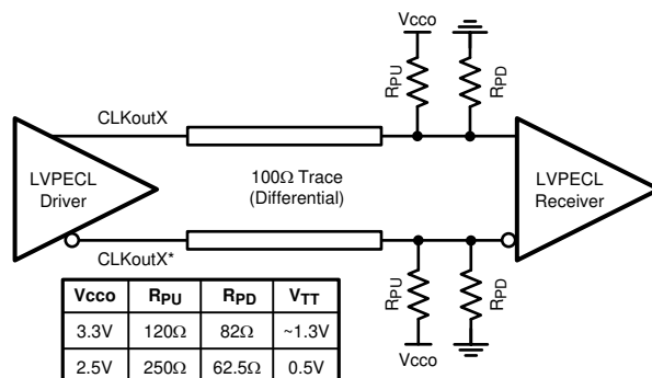
图 10-9. Differential LVPECL Operation, DC Coupling, Thevenin Equivalent
