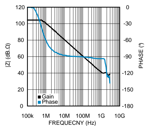
Figure 22. Open Loop Transimpedance
