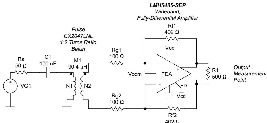
图 9-2. Input Balun Interface Delivers a Differential Input to the LMH5485-SEP
