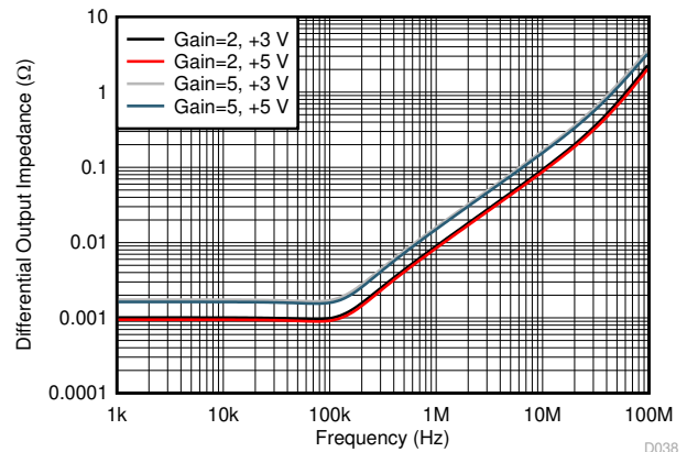
图 7-10. Closed-Loop Output Impedance
