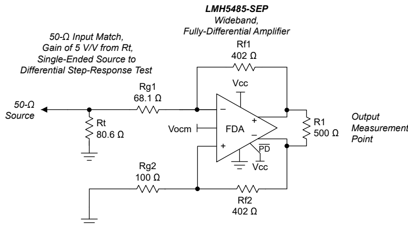
图 8-2. DC-Coupled, Single-Ended-to-Differential, Basic Test Circuit Set for a Gain of 5 V/V
