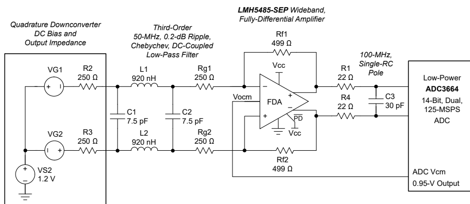
图 9-3. Example DC-Coupled, Differential I/O Design from a Quadrature Mixer to an ADC
