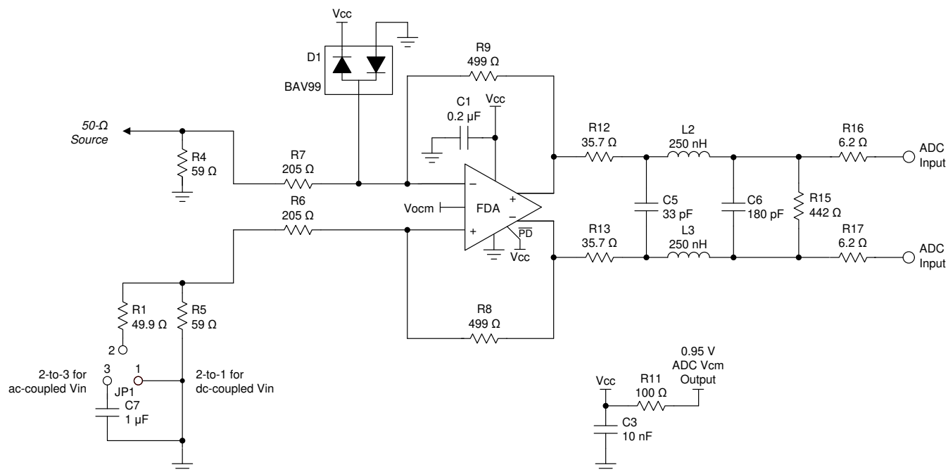
图 10-4. DC-Coupled, Bipolar Input Gain of 2 V/V Single-Ended to Differential Interface to ADC
