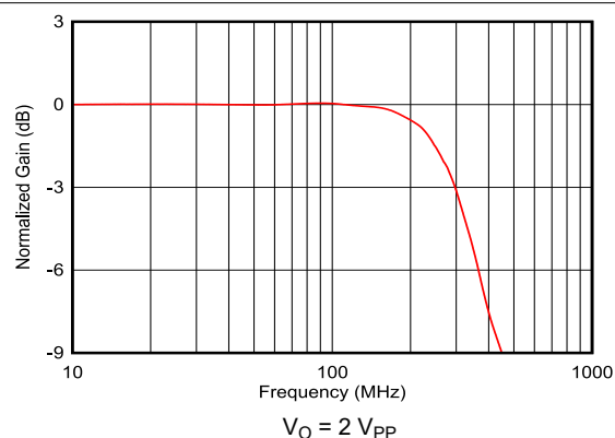
图 7-2. Large-Signal Frequency Response
