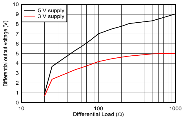
图 7-21. Differential Output Voltage vs Rload
