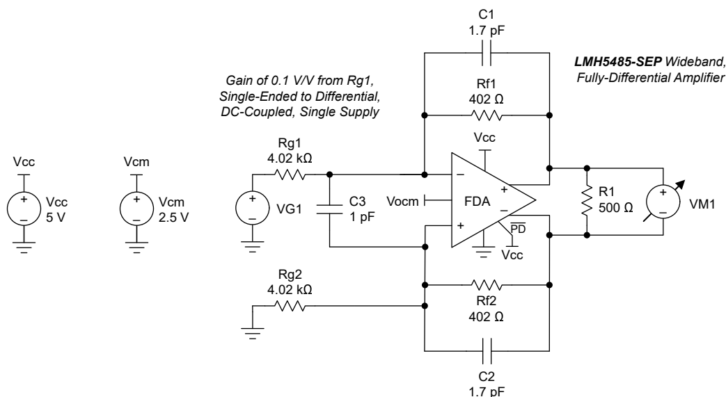
图 10-2. Compensated Attenuator Circuit Using the LMH5485-SEP
