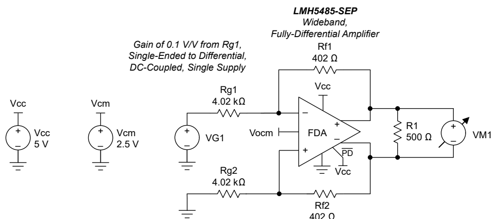
图 10-1. Divide-by-10 Attenuator Application for the LMH5485-SEP
