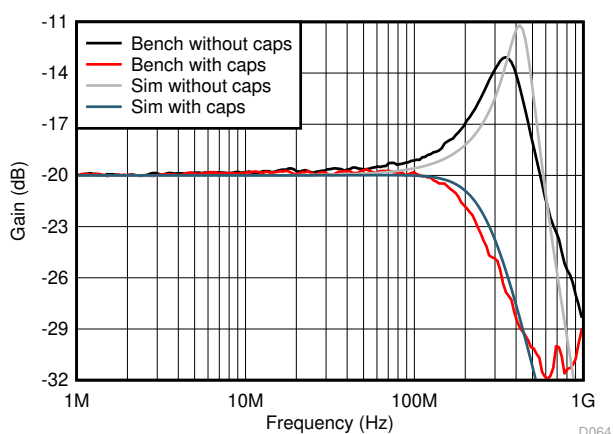
图 10-3. Attenuator Response Shapes with and without External Compensation
