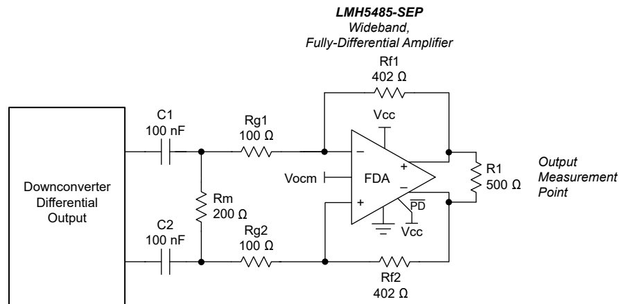
图 9-1. Down-Converter Mixer Delivering an AC-Coupled Differential Signal to the LMH5485-SEP
