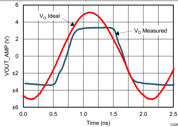
图 31. SE-DE Output Common Mode Pulse Response
