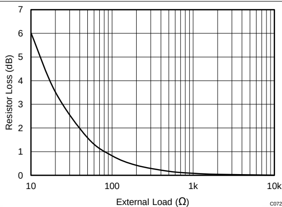
图 76. Gain Loss Resulting from On-Chip Output Resistors
