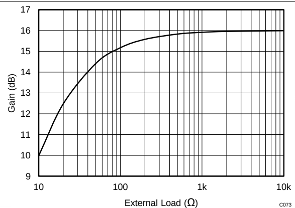
图 77. Net Gain versus Load Resistance
