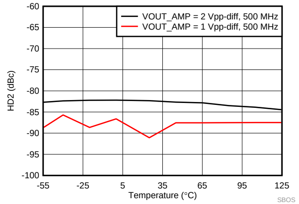
图 20. SE-DE 2nd Order Harmonic Distortion vs Temperature
