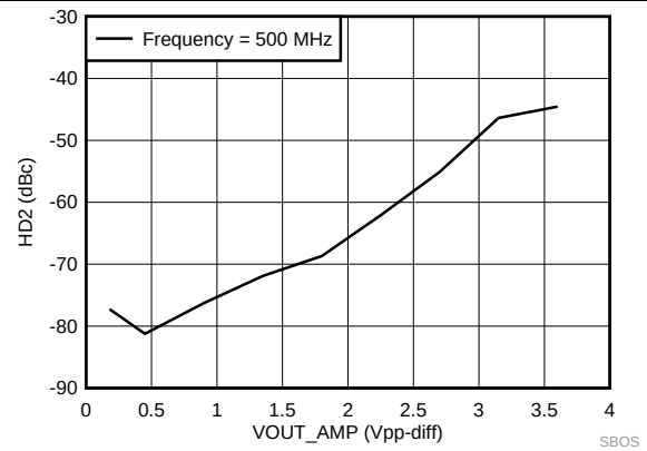
图 41. SE-DE 2nd Order Harmonic Distortion vs Vout
