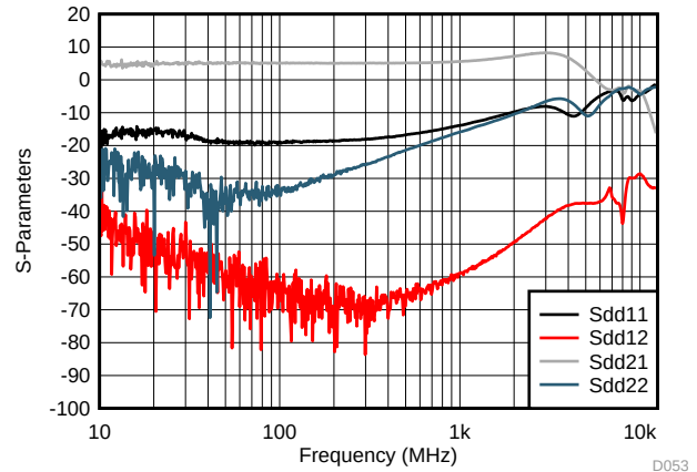
图 8. DIFF-DIFF Small Signal S-Parameters
