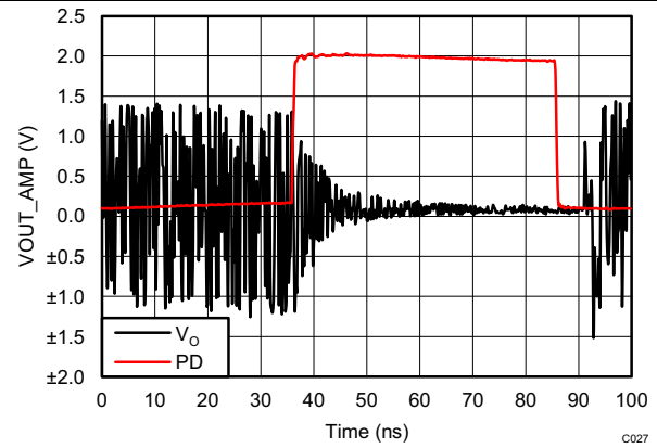
图 32. Power Down Timing
