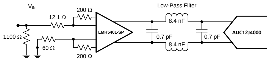
图 65. Low-Loss ADC
