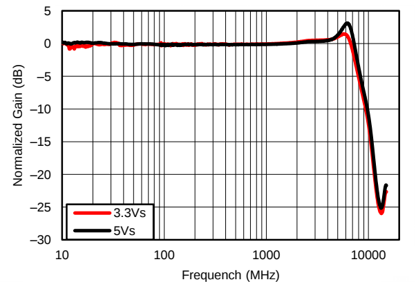
Figure 2. Frequency Response Differential Input
