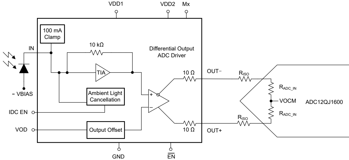
图 8-2. LMH32404-Q1 (Single Channel) to ADC Interface With a Matching Resistor Network
