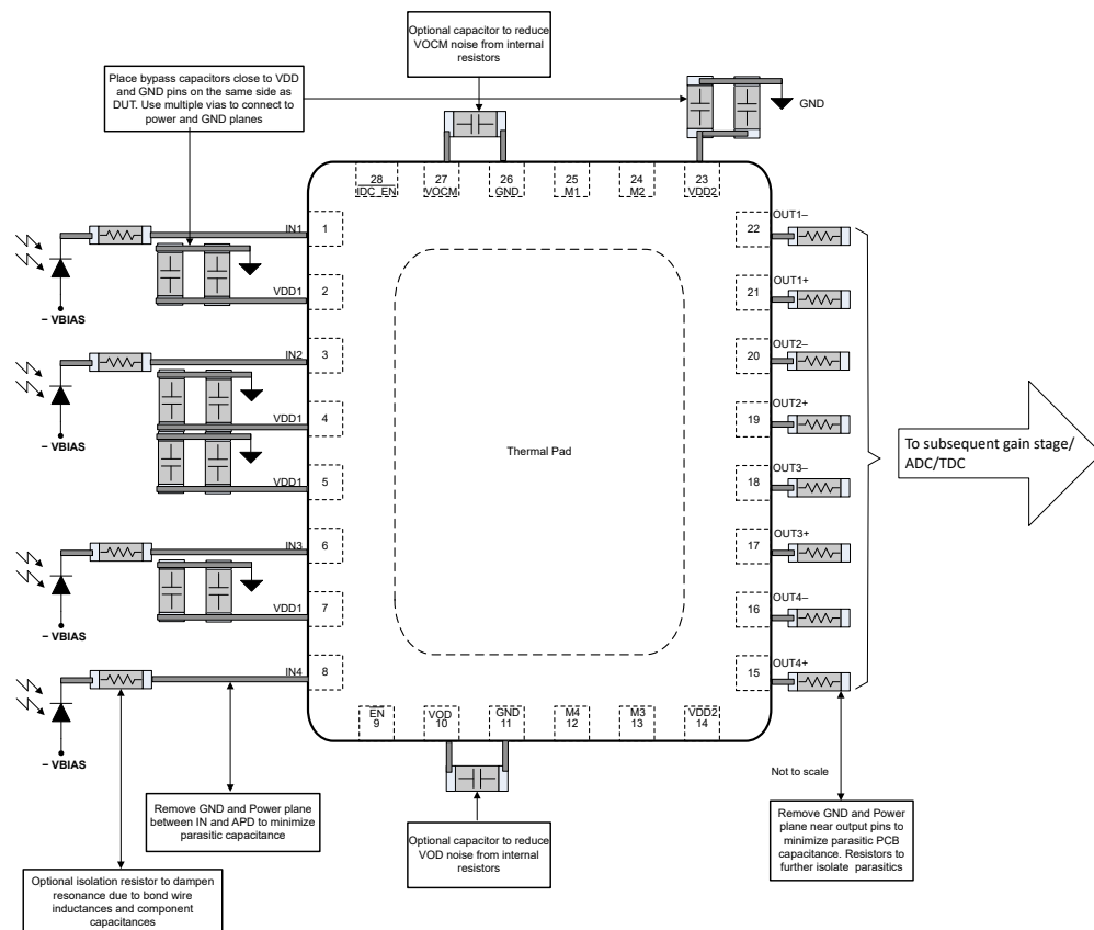
图 10-1. Layout Recommendation
