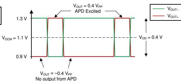
图 7-2. Single-Ended Outputs With VOD = 0.4 V
