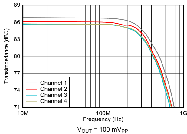
图 6-3. Small Signal Response vs Channels
