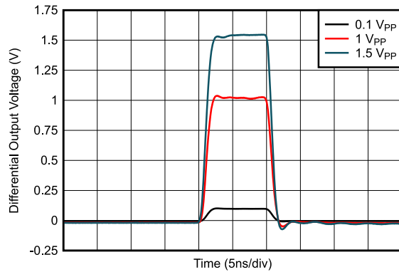
图 6-13. Pulse Response vs Output Swing
