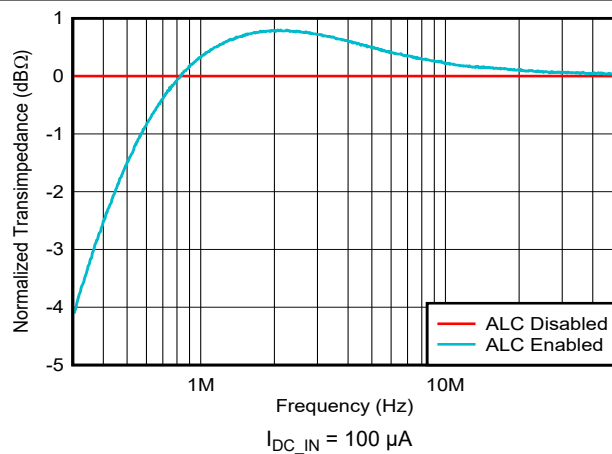
图 6-5. Low-Side Frequency Response vs Ambient Light Cancellation
