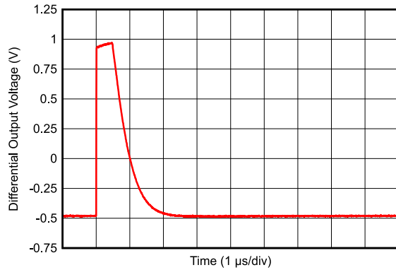
图 6-19. Ambient Loop Cancellation Settling Time (1)
