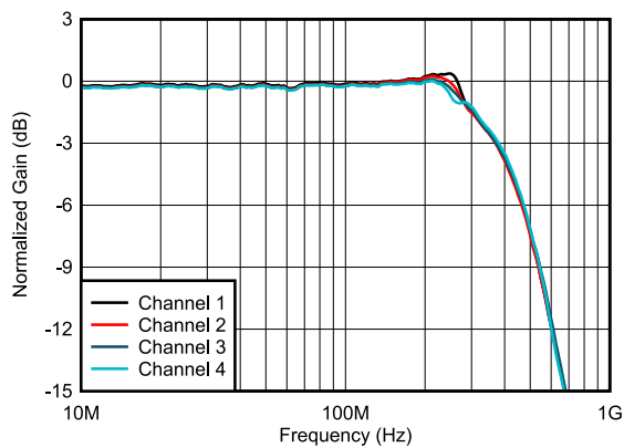
图 8-5. Transimpedance Bandwidth
