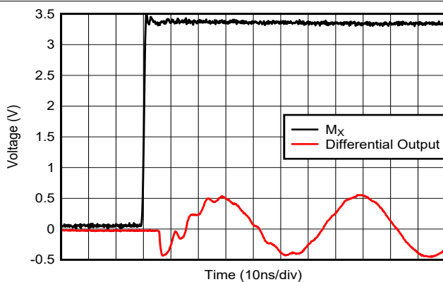
图 8-7. Channel Turn-On Response
