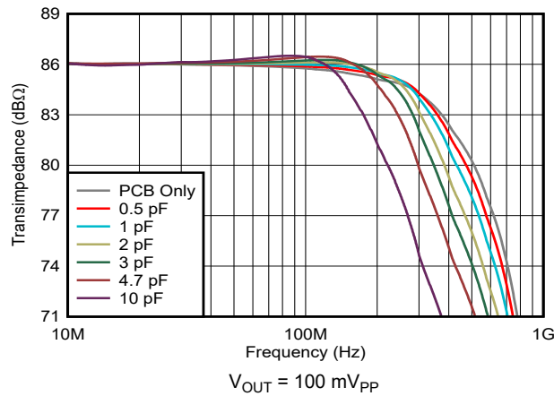
图 6-1. Small Signal Response vs Input Capacitance
