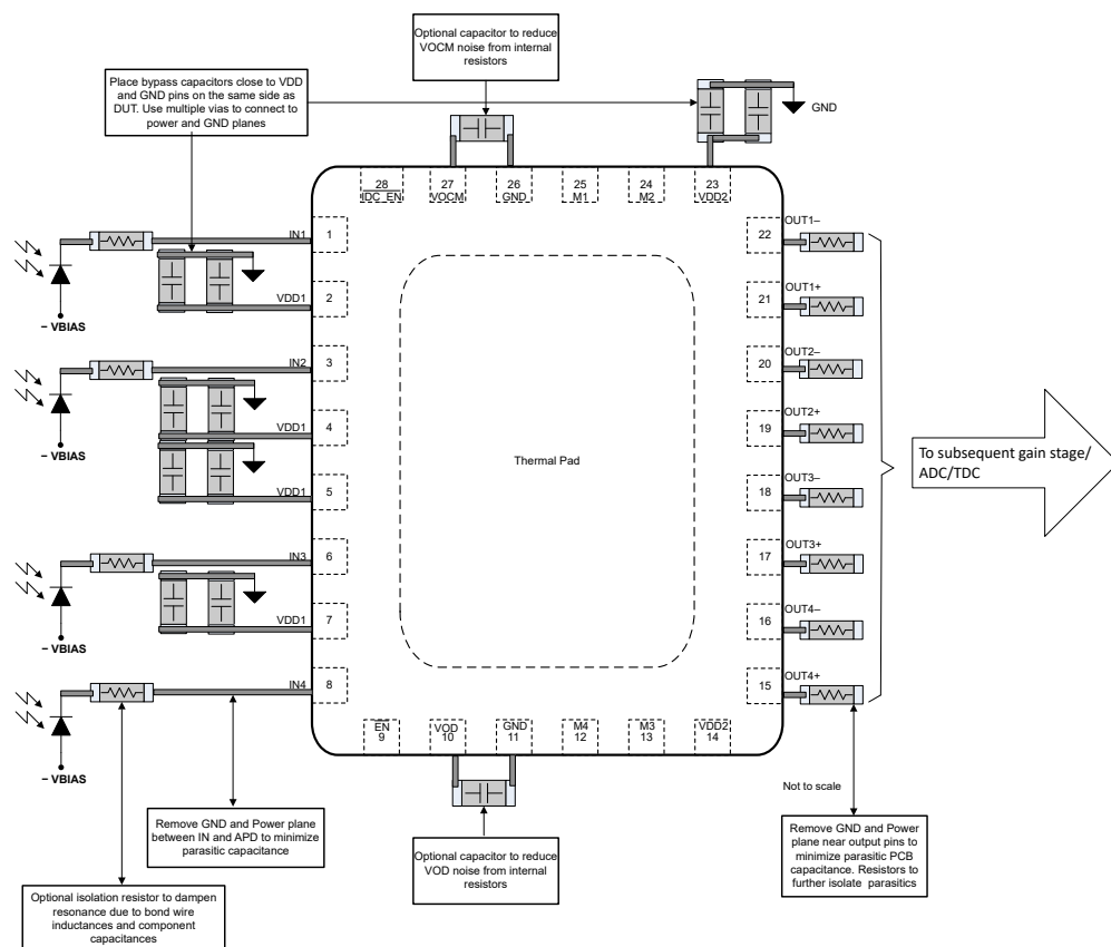
图 10-1. Layout Recommendation
