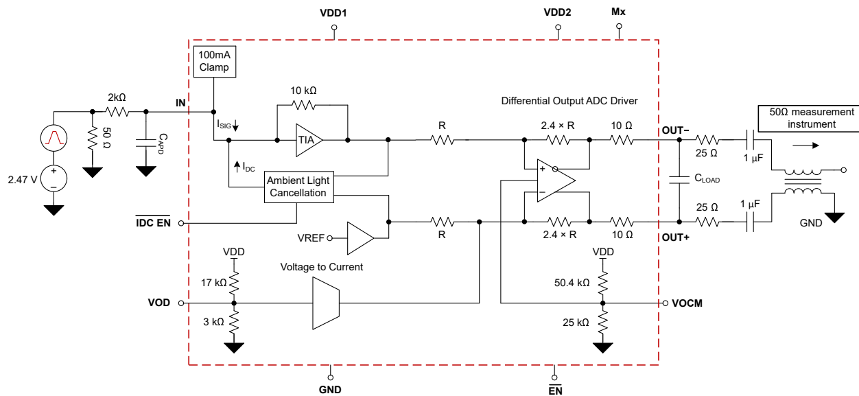
图 8-3. LMH32404 Single Channel Test Circuit for Single-Ended Measurement
