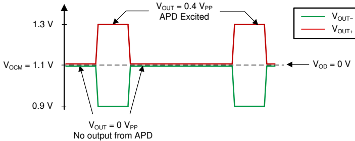
图 7-1. Single-Ended Outputs With VOD = 0 V
