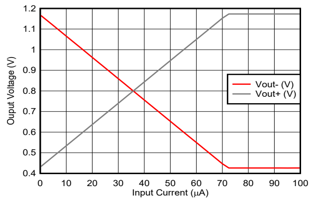
图 6-28. Low-Side Swing vs Input Current
