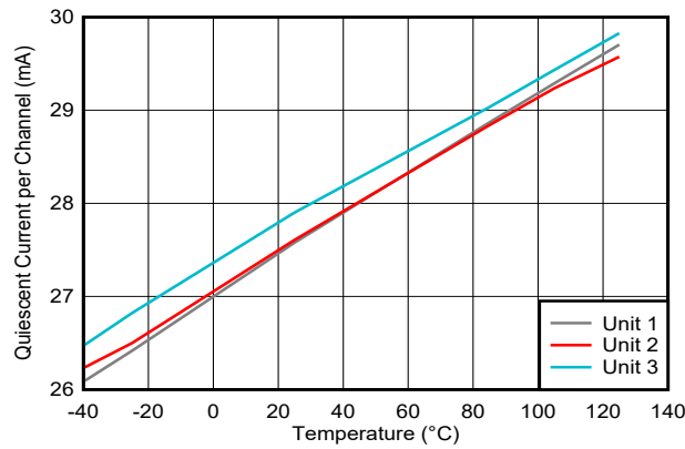
图 6-25. Quiescent Current (Per Channel) vs Ambient Temperature (2)
