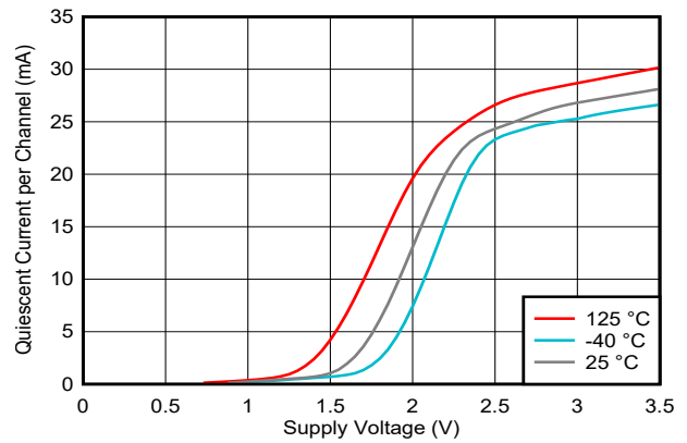
图 6-26. Quiescent Current (Per Channel) vs Supply Voltage
