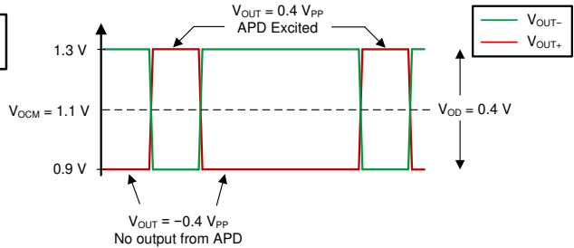
图 7-2. Single-Ended Outputs With VOD = 0.4 V
