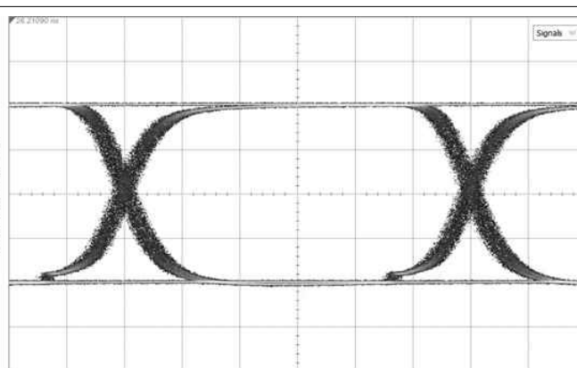
图 9-12. 1.485 Gbps, TL = 20" FR4, Reclocked
