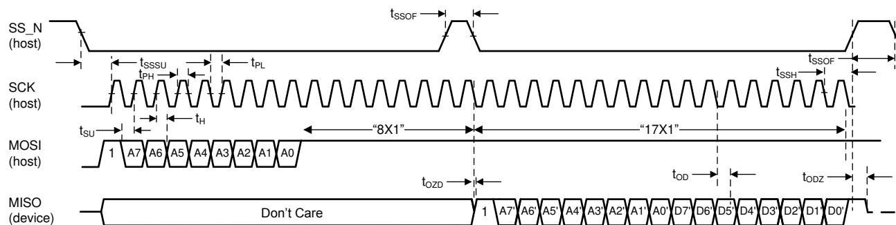
图 8-10. Signal Timing for a SPI Read Transaction
