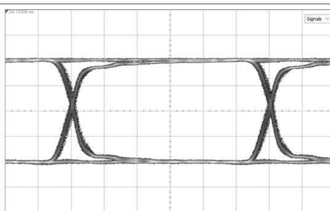
图 9-18. 5.94 Gbps, CC = 120-m Belden 1694A, Reclocked
