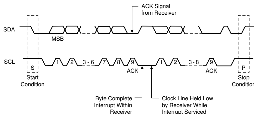
图 8-5. Acknowledge (ACK)
