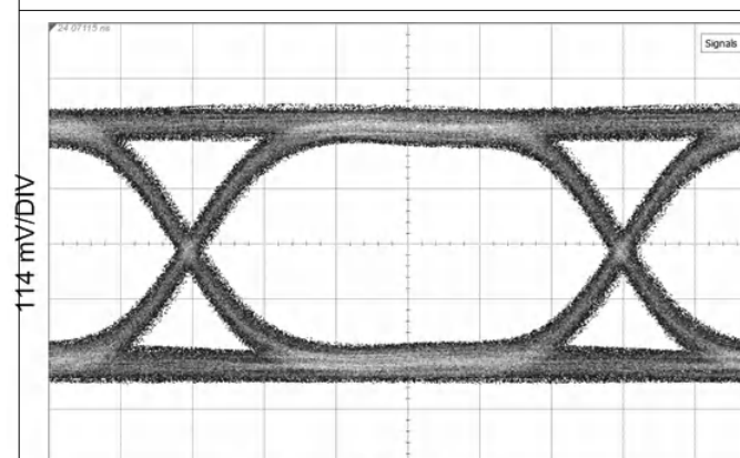
图 9-5. 11.88 Gbps, CC = 75-m Belden 1694A, Reclocked
