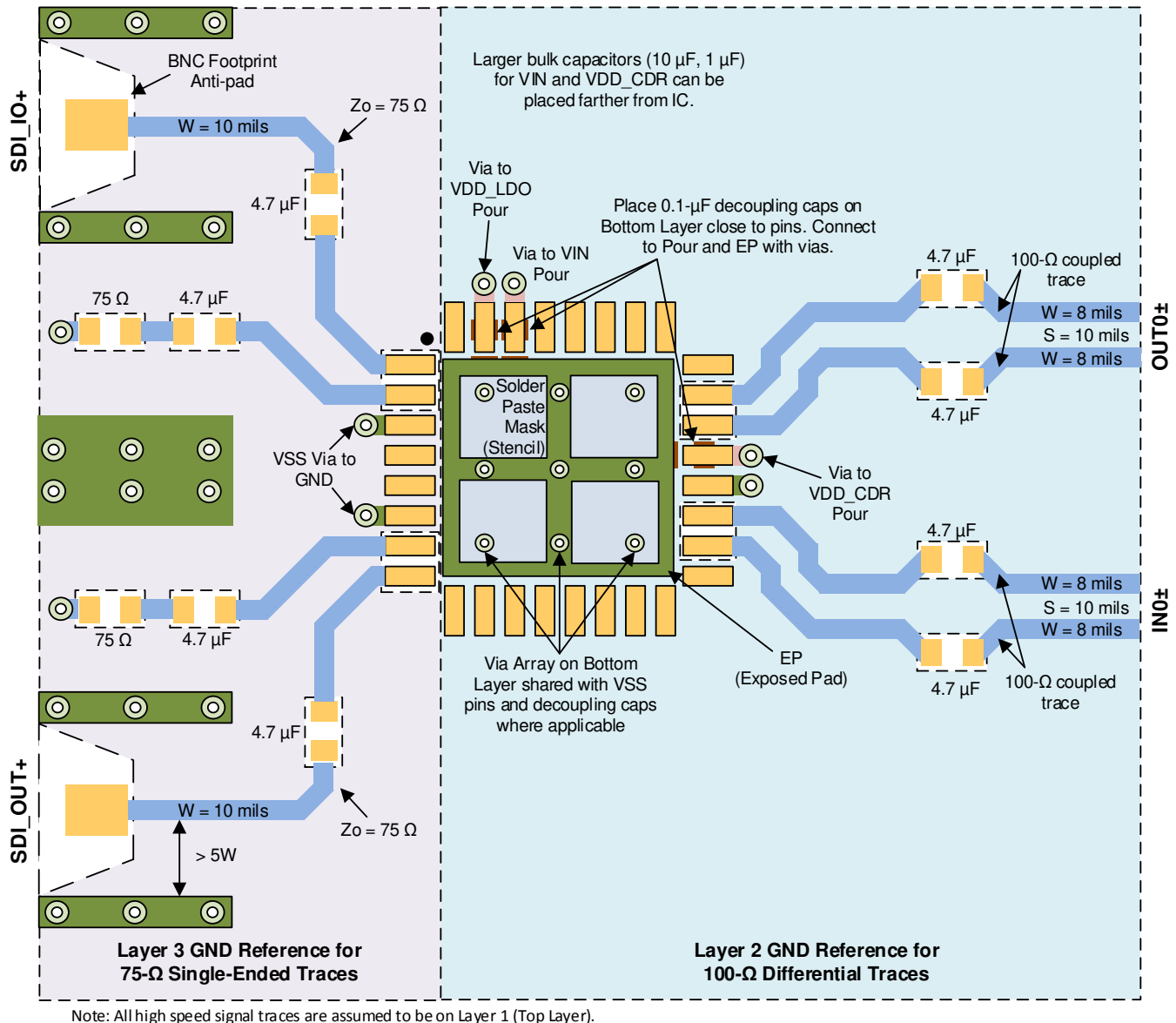
图 11-1. LMH1297 High-Speed Trace Layout Example
