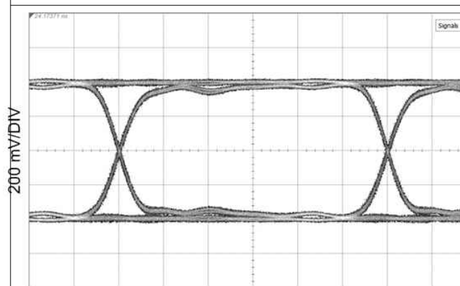
图 9-17. 11.88 Gbps, CC = 65-m Belden 1694A, Reclocked
