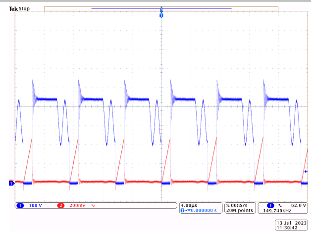
图 8-3. V_{IN} = 230VAC V_{OUT} = 20V I_{OUT} = 3.25A
