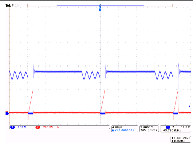
图 8-5. V_{IN} = 230VAC V_{OUT} = 5V I_{OUT} = 3A
