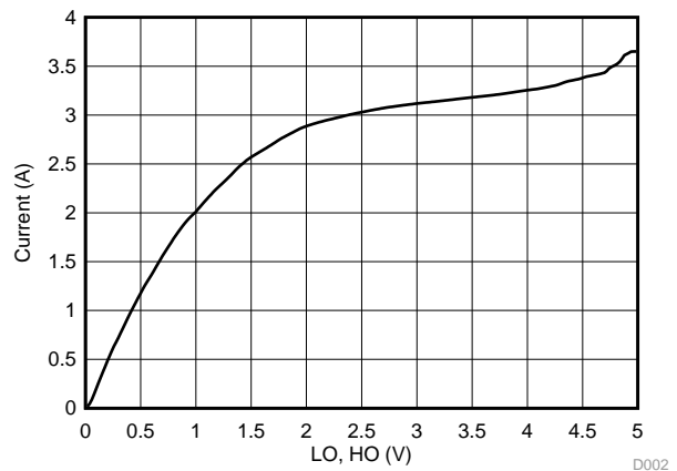
图 2. Peak Sink Current vs Output Voltage
