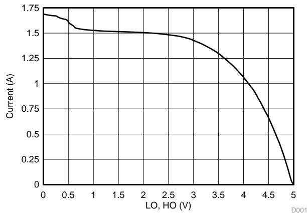
图 1. Peak Source Current vs Output Voltage
