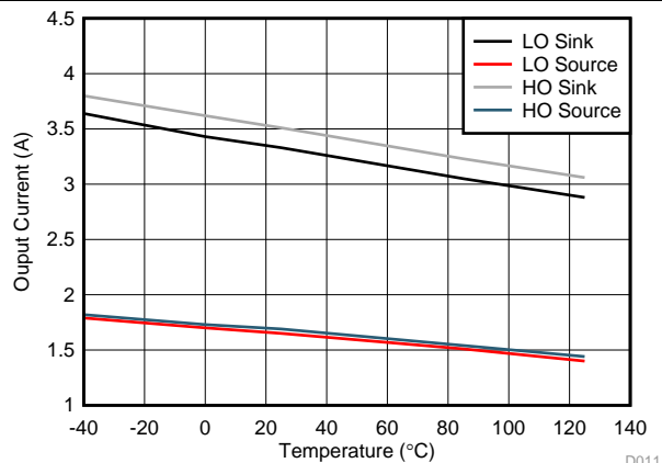
图 11. LO and HO Output Current vs Temperature
