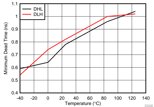
图 8. Minimum Dead Time vs Temperature
