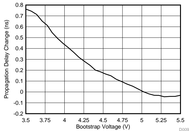
图 9. Propagation Delay Change vs Bootstrap voltage
