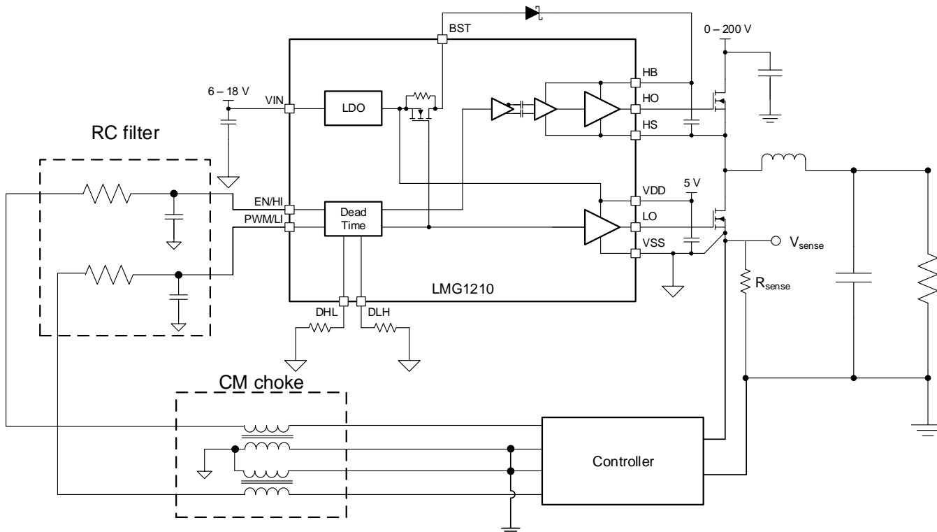
图 18. LMG1210 Configured With Current Sense Resistor Using a CMC as Filter
