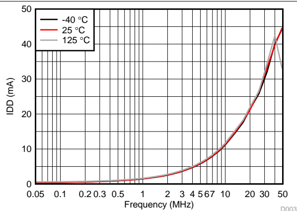
图 3. IDD vs Frequency, Unloaded
