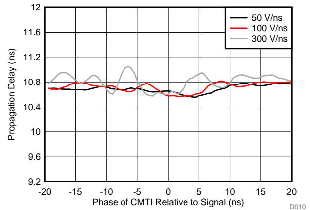
图 10. Propagation Delay vs relative phase of CMTI Phase
