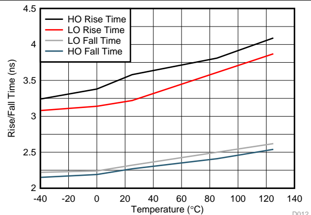
图 12. 1 nF Loaded Rise and Fall Time vs Temperature
