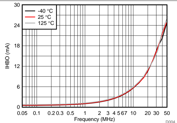
图 4. I_{HBO} vs Frequency, Unloaded
