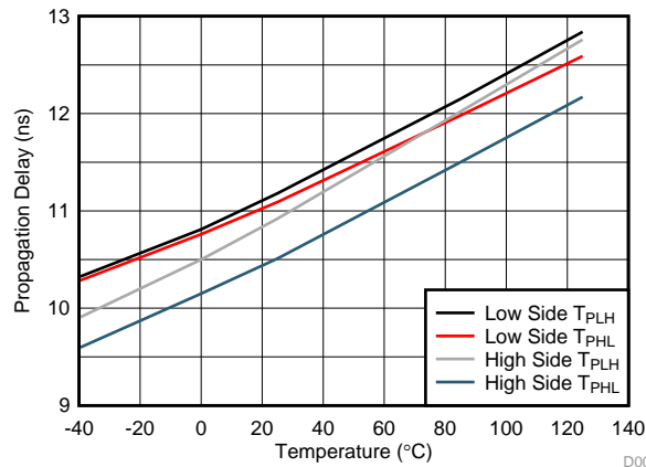
图 7. Propagation Delay vs Temperature
