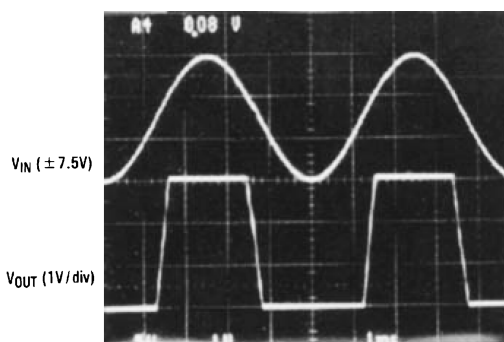
Figure 54. A \pm 7.5V Input Signal Greatly Exceeds the 3V Supply in Figure 55 Causing No Phase Inversion Due to R_i
