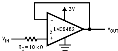
Figure 55. R_T Input Current Protection for Voltages Exceeding the Supply Voltages
