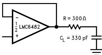
Figure 56. Resistive Isolation of a 330pF Capacitive Load
