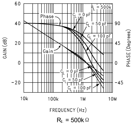
图 5-15. Gain and Phase Response vs Capacitive Load
