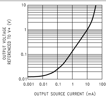
图 5-7. Output Characteristics Current Sourcing
