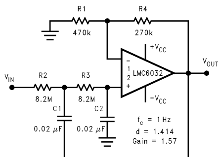
图 6-13. 1Hz Low-Pass Filter (Maximally Flat, Dual Supply Only)
