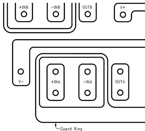
图 6-16. Example of Guard Ring in PCB Layout
