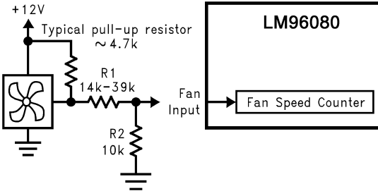
Figure 16. Fan with Tach Pull-Up to +12V, or Totem-Pole Output and Resistor Attenuator
