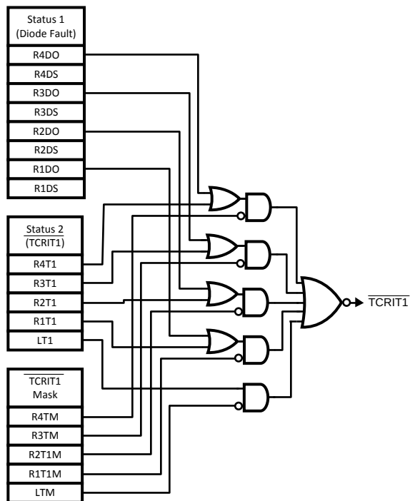
Figure 15. \overline{\text{TCRIT1}} Mask Register, Status Register 1 and 2, and TCRIT1 output logic diagram.
