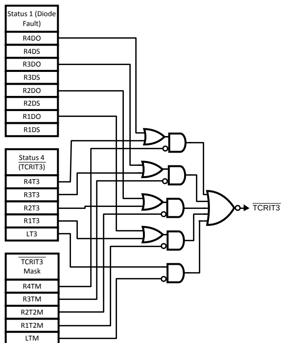
Figure 17. \overline{\text{TCRIT3}} Mask Register, Status Register 1 and 4, and TCRIT3 output logic diagram.
