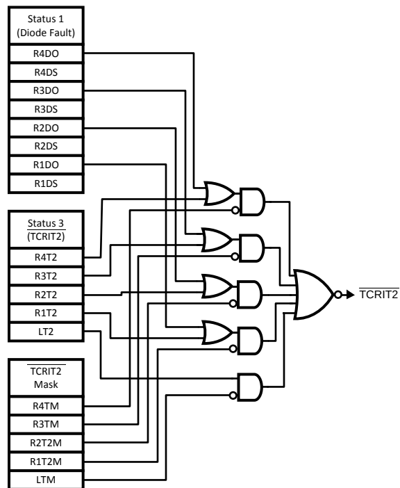
Figure 16. \overline{\text{TCRIT2}} Mask Register, Status Register 1 and 3, and TCRIT2 output logic diagram.
