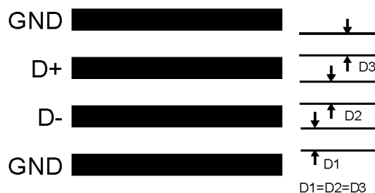
Figure 18. Ideal Diode Trace Layout
