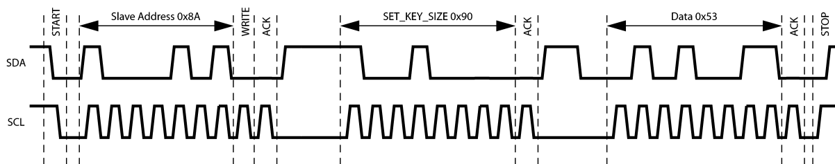
Figure 18. Host Write Command
