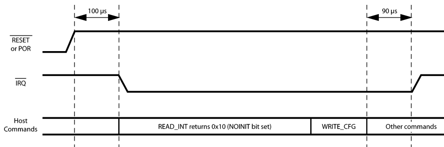
Figure 5. IRQ Reset Timing
