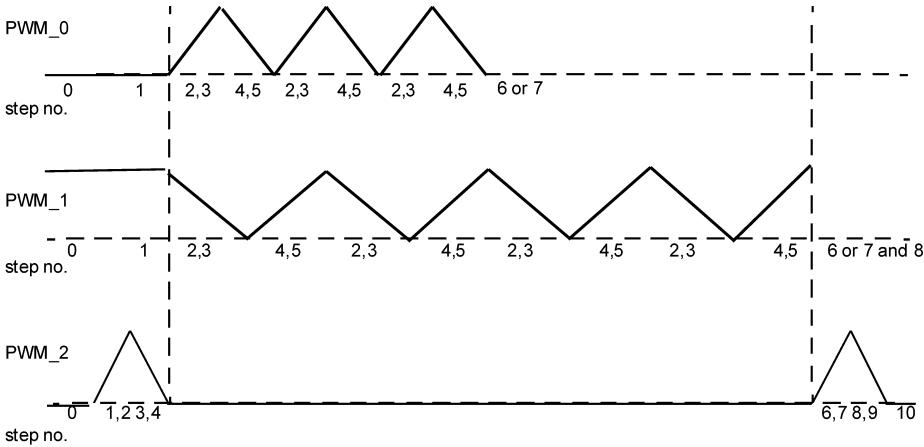
Figure 16. PWM Outputs
