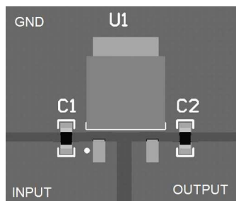
Figure 17. Layout Recommendation
