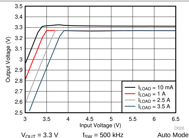
图 51. LM76003 Dropout Curve
