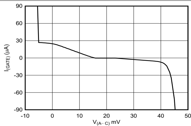
图 6-11. Gate Current vs Forward Voltage Drop
