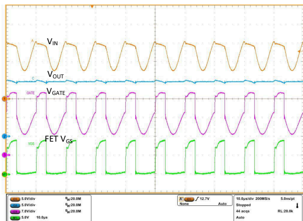
图 9-3. AC Super Imposed Test - 6-V Peak-Peak 100 kHz
