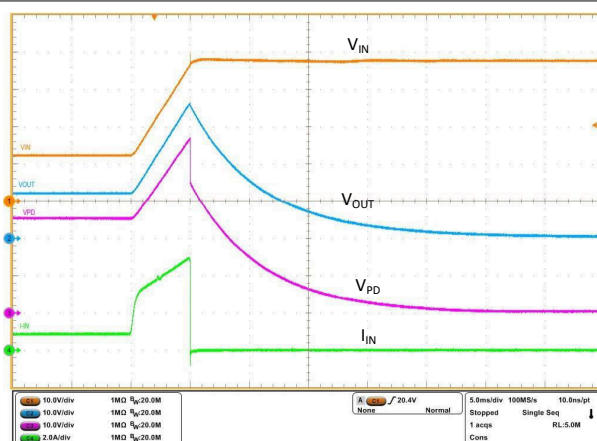
图 9-16. Overvoltage Protection
